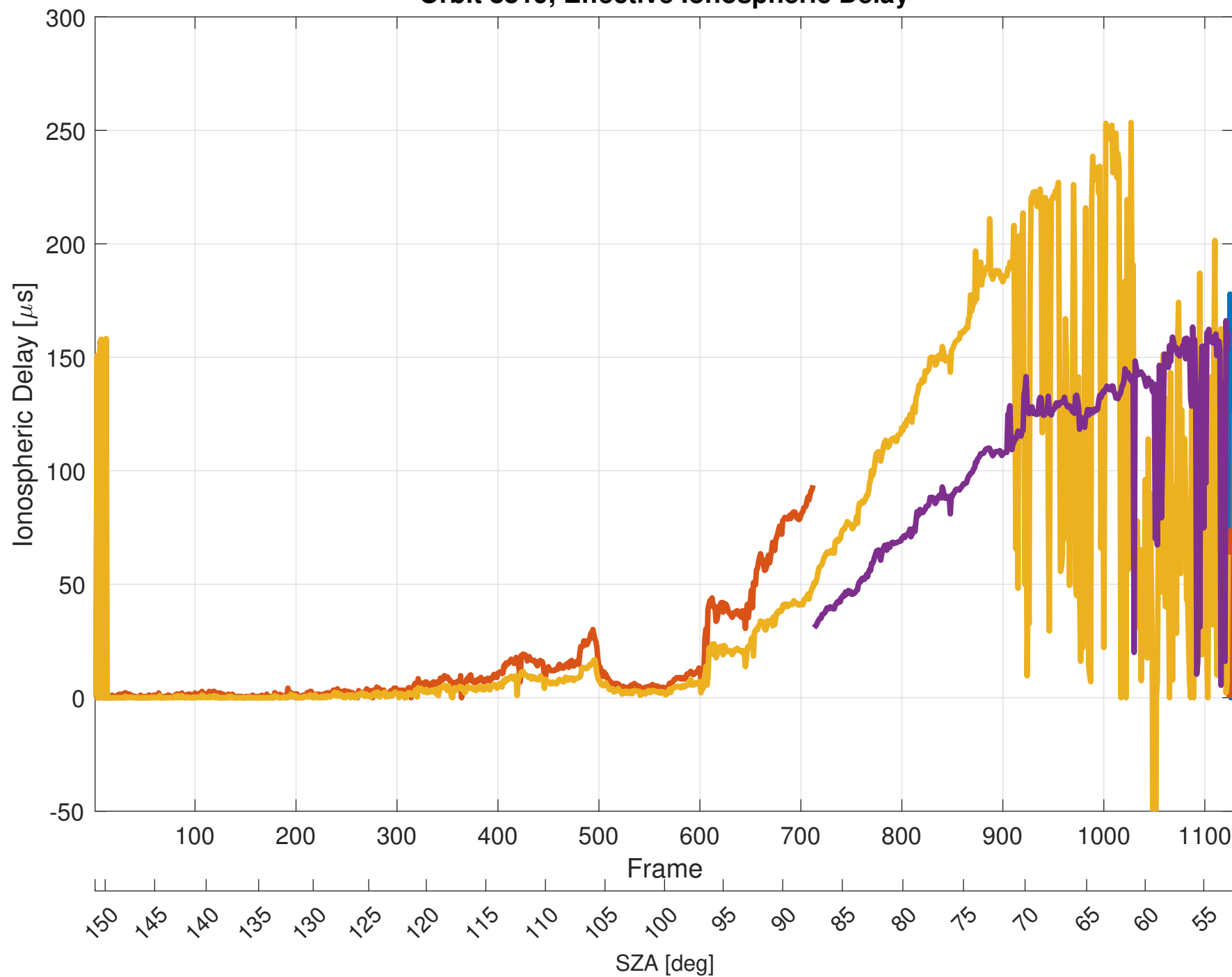
Orbit 8819, Effective Ionospheric Delay
