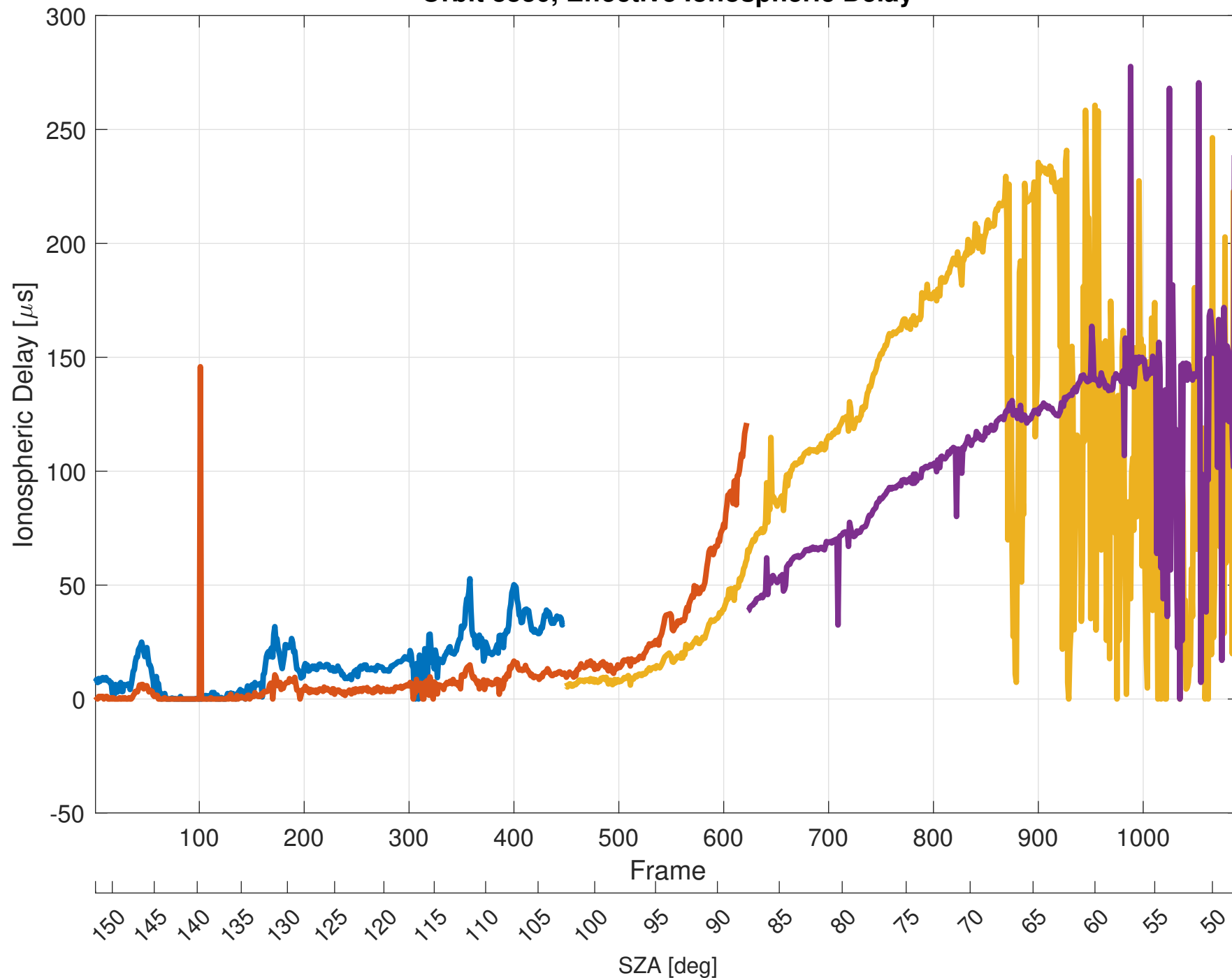
Orbit 8830, Effective Ionospheric Delay
