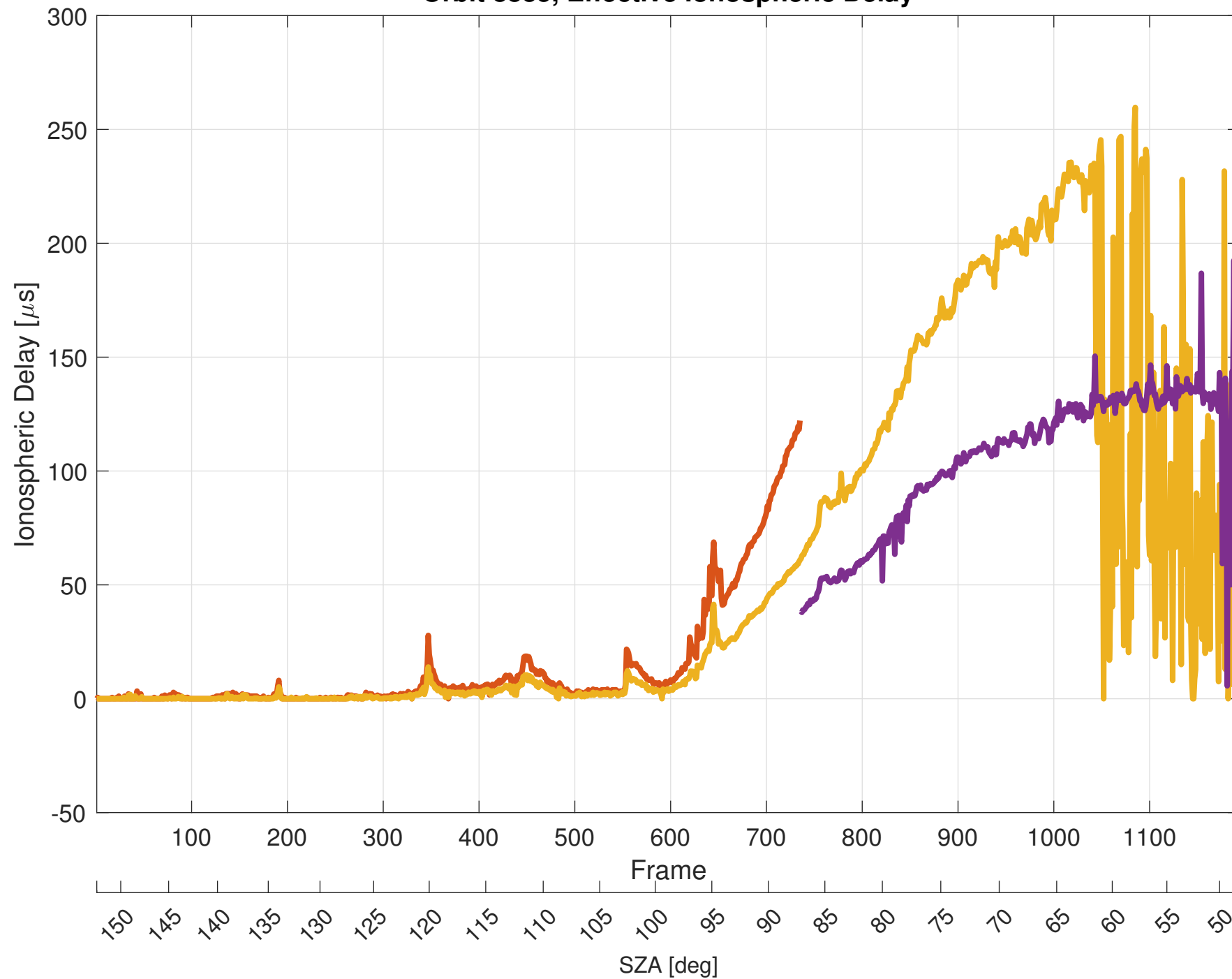
Orbit 8835, Effective Ionospheric Delay
