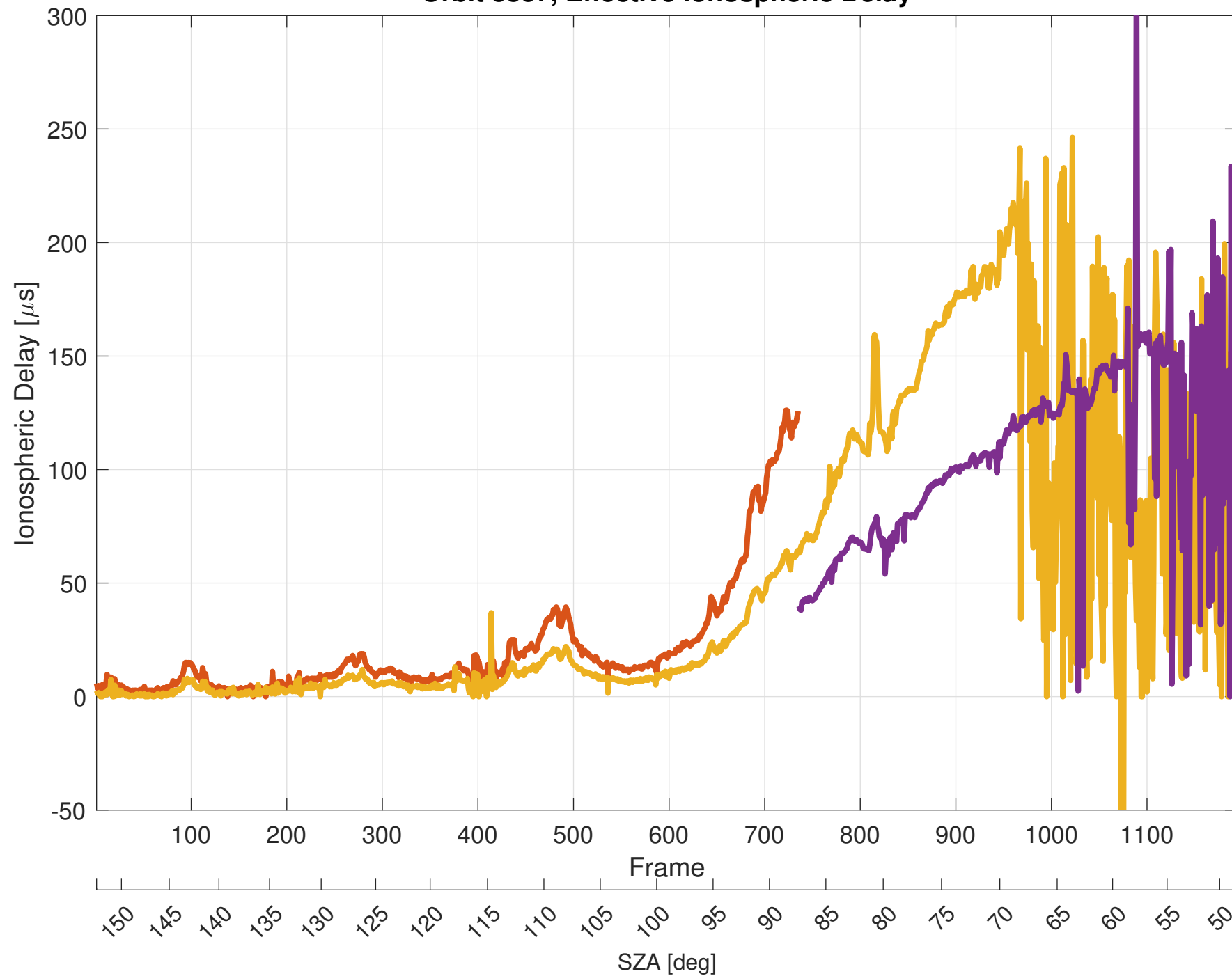
Orbit 8837, Effective Ionospheric Delay
