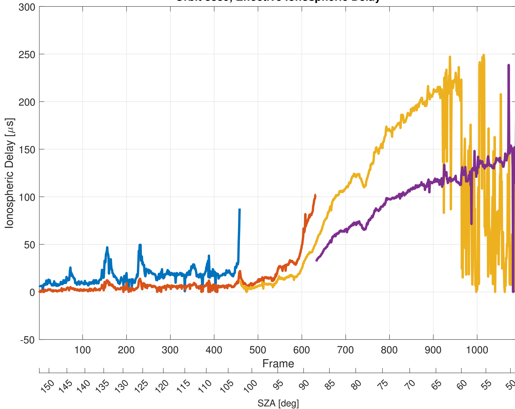
Orbit 8839, Effective Ionospheric Delay
