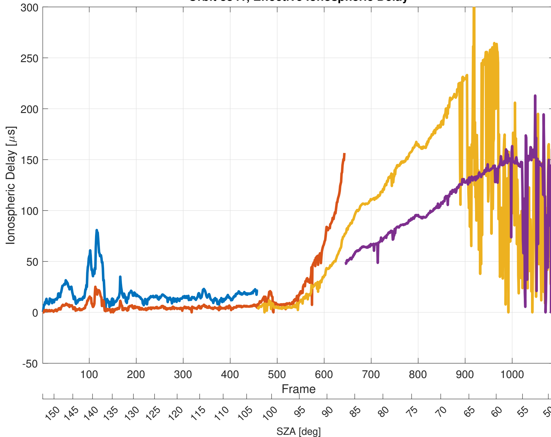
Orbit 8841, Effective Ionospheric Delay
