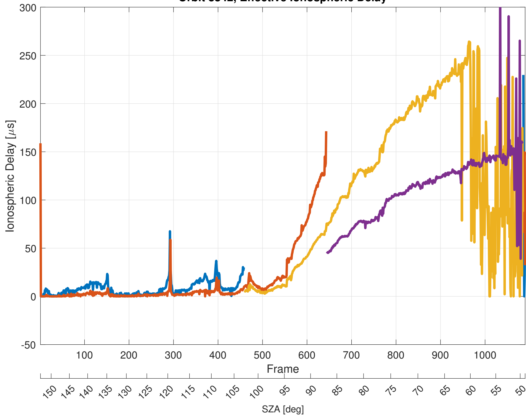
Orbit 8842, Effective Ionospheric Delay
