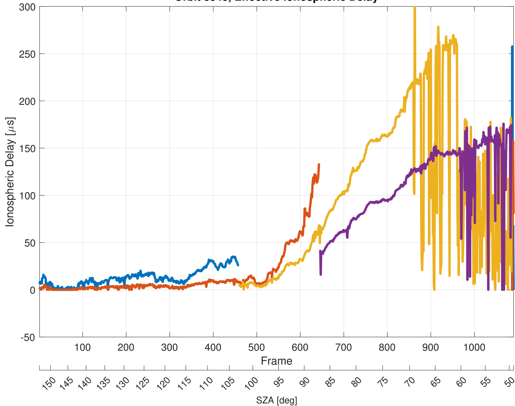
Orbit 8843, Effective Ionospheric Delay
