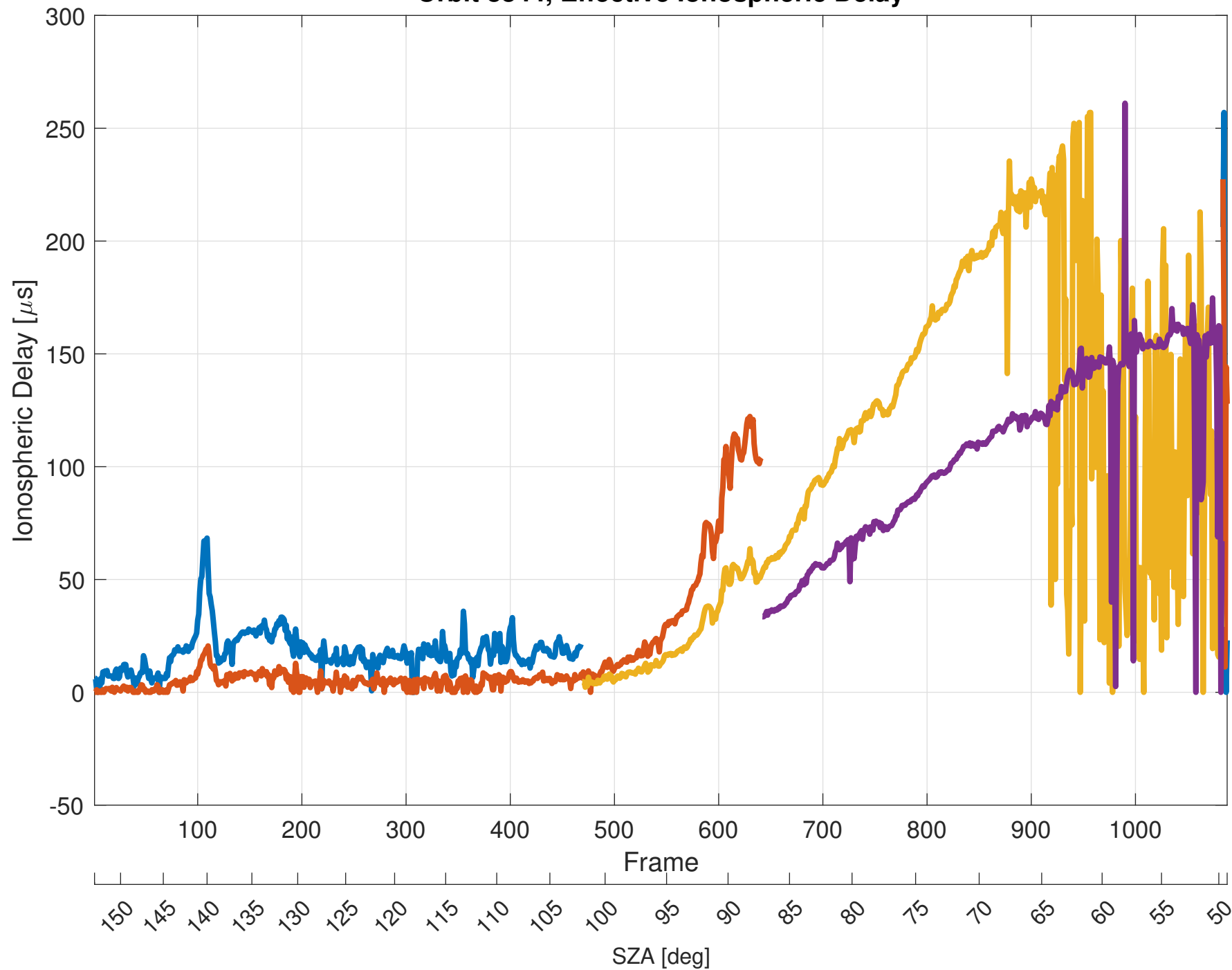
Orbit 8844, Effective Ionospheric Delay
