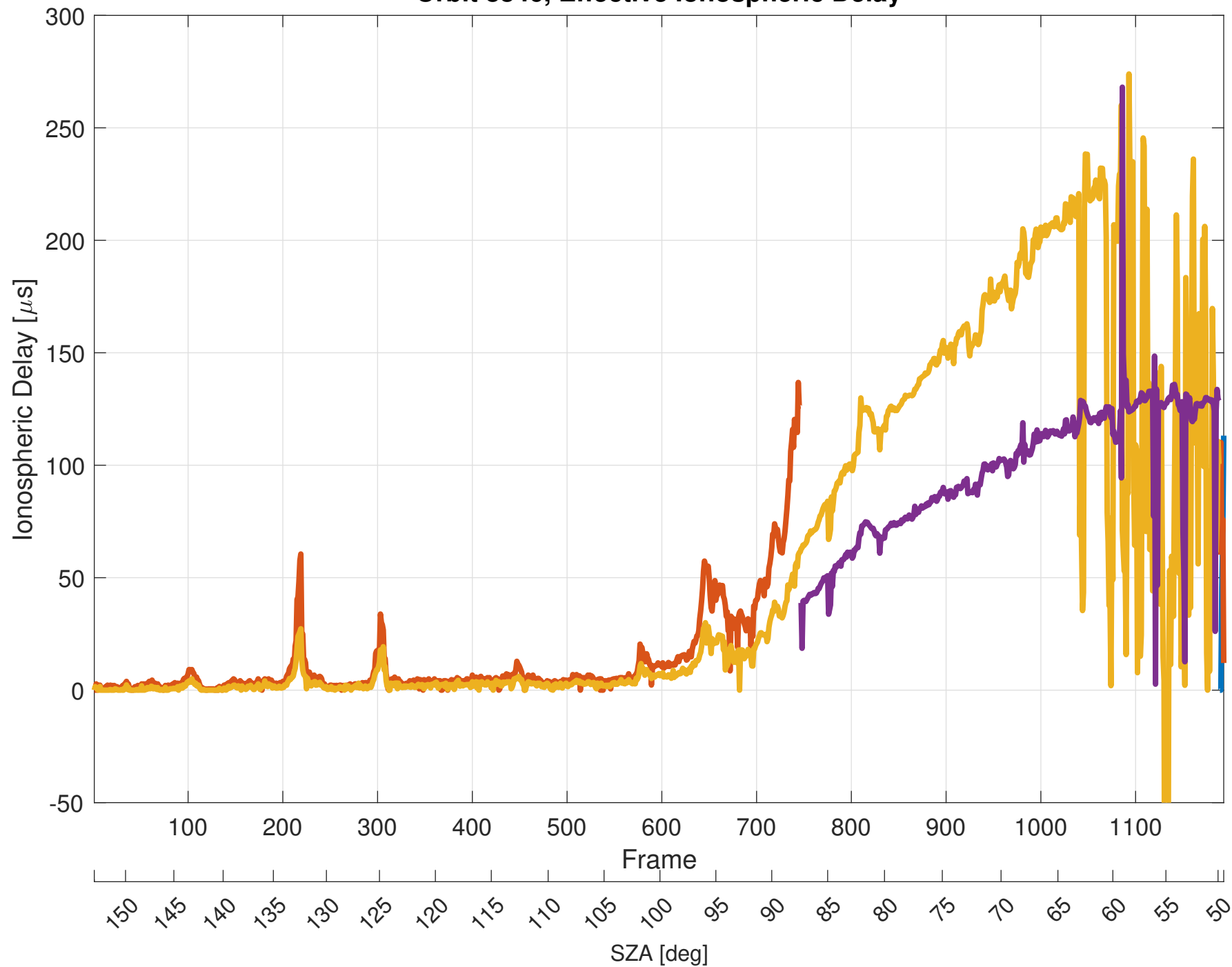
Orbit 8846, Effective Ionospheric Delay
