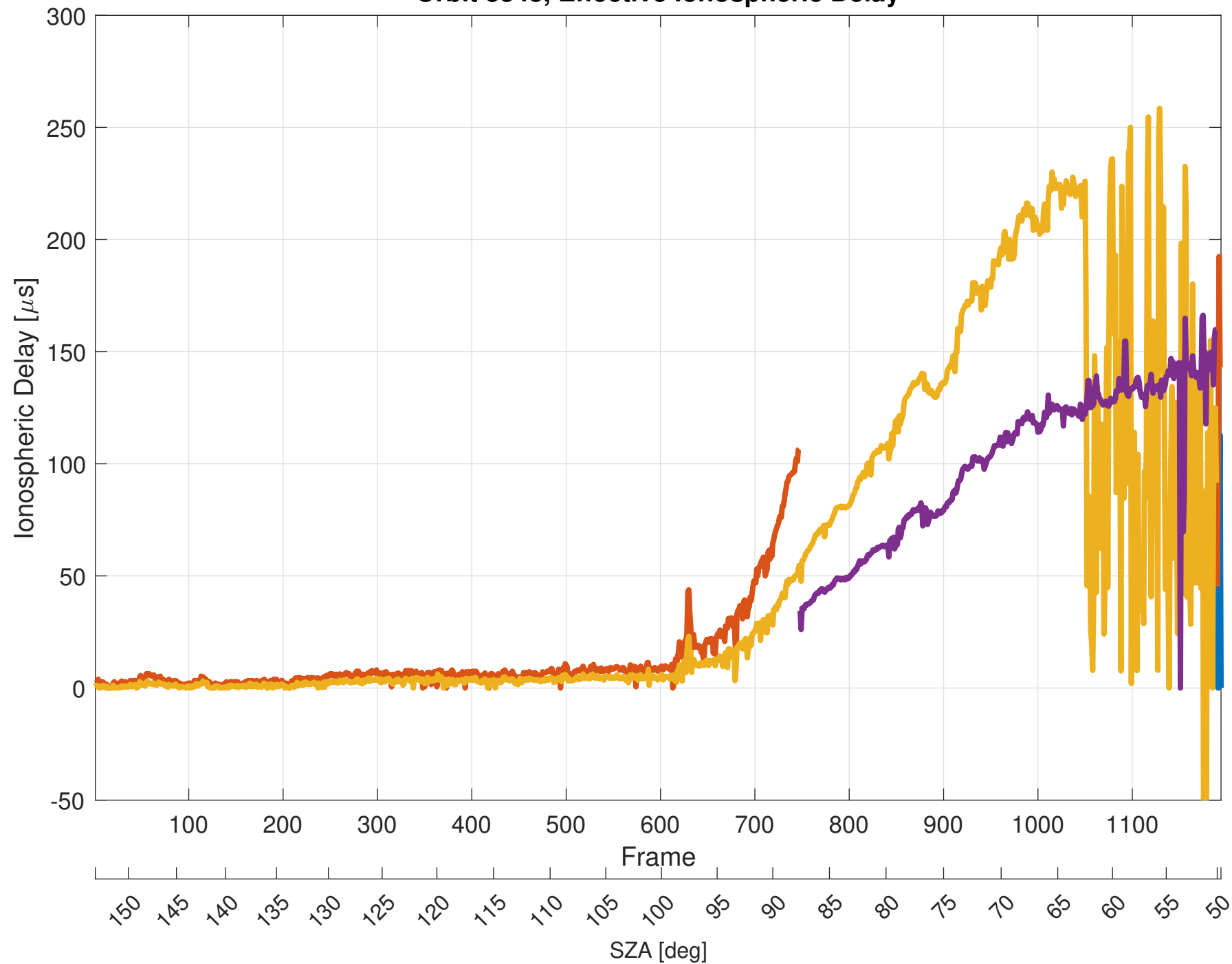
Orbit 8848, Effective Ionospheric Delay
