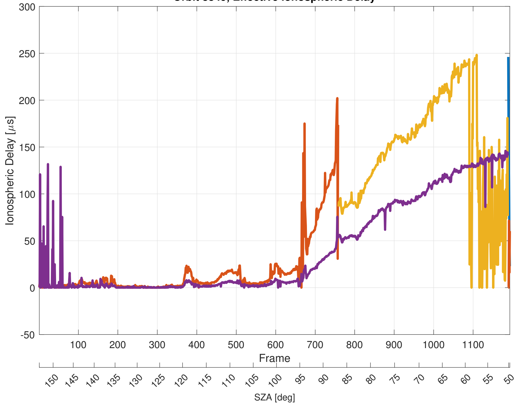
Orbit 8849, Effective Ionospheric Delay
