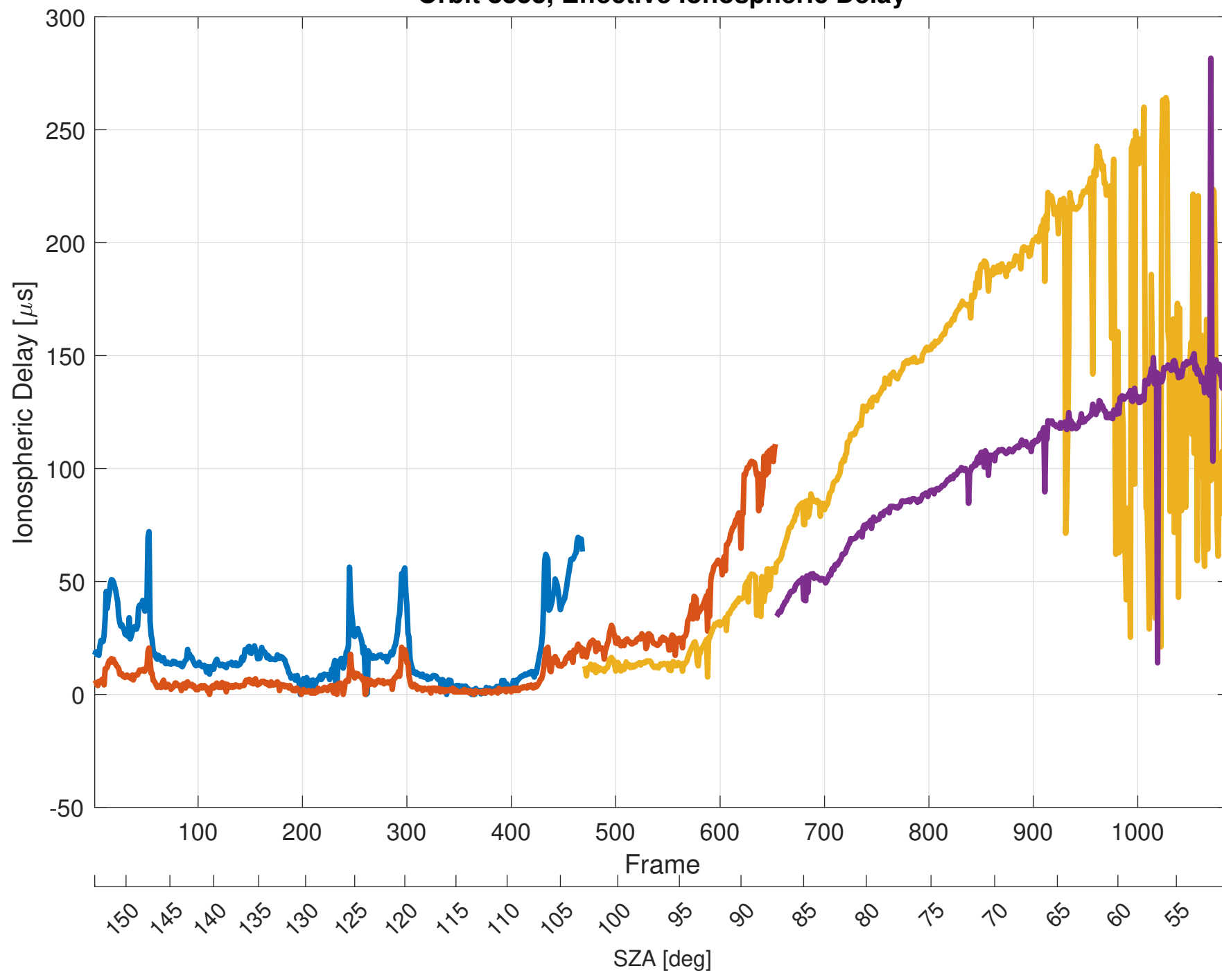
Orbit 8853, Effective Ionospheric Delay
