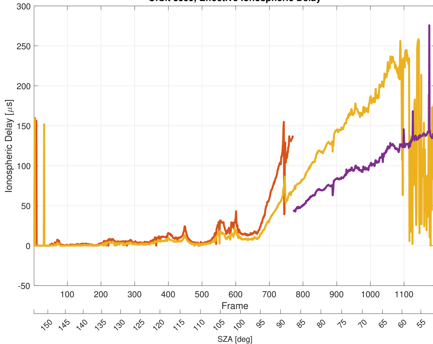
Orbit 8859, Effective Ionospheric Delay
