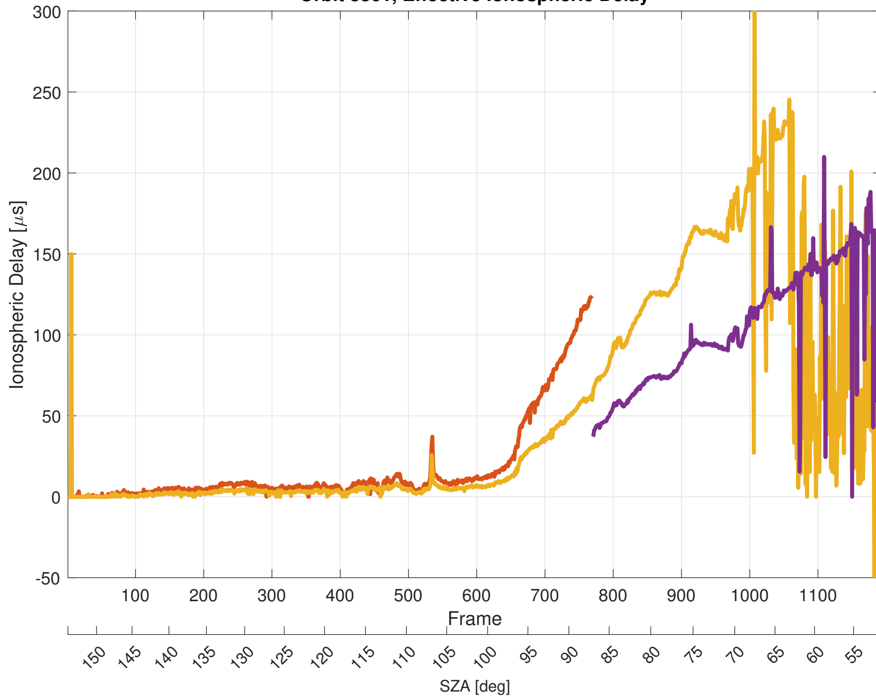
Orbit 8861, Effective Ionospheric Delay
