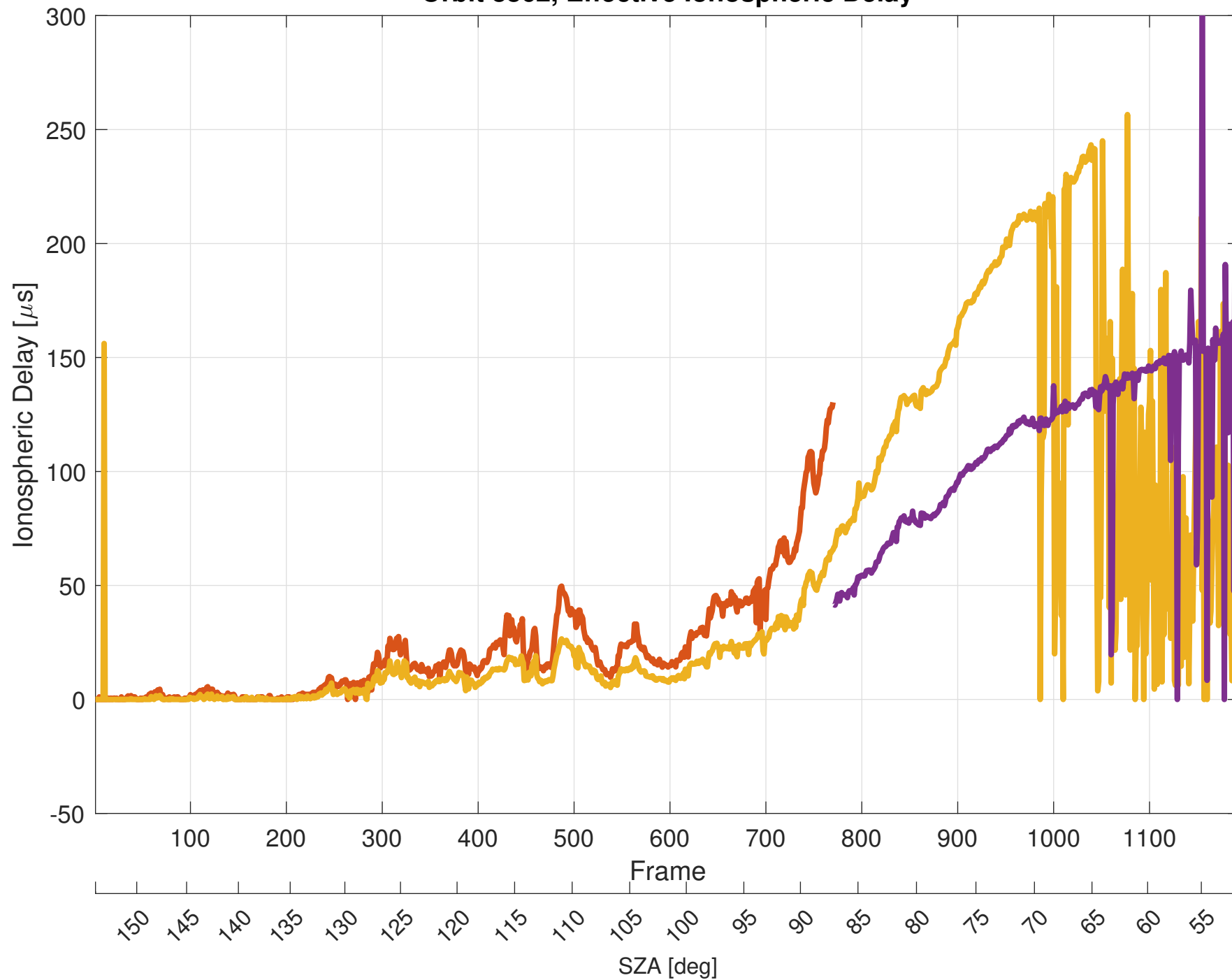
Orbit 8862, Effective Ionospheric Delay
