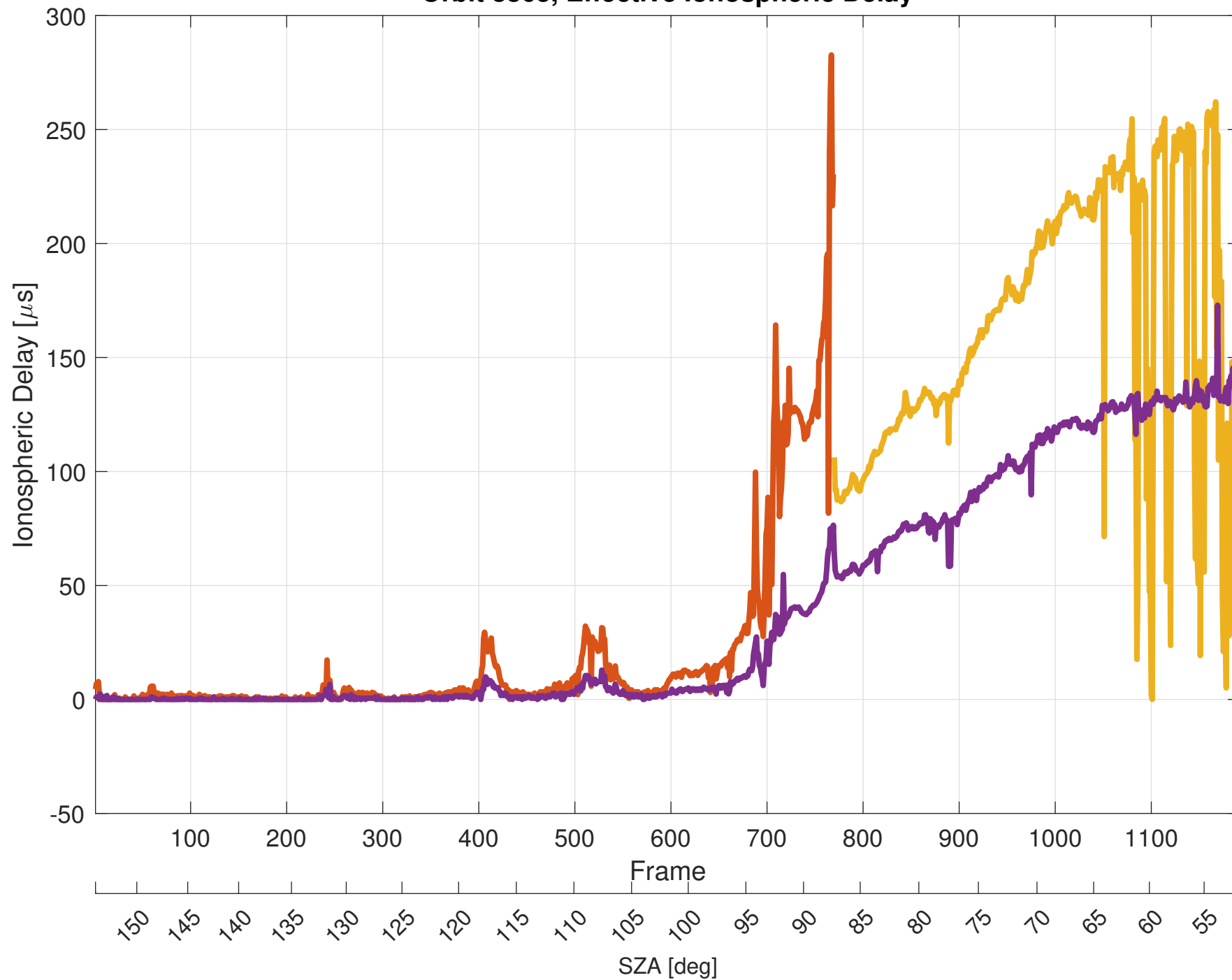
Orbit 8863, Effective Ionospheric Delay
