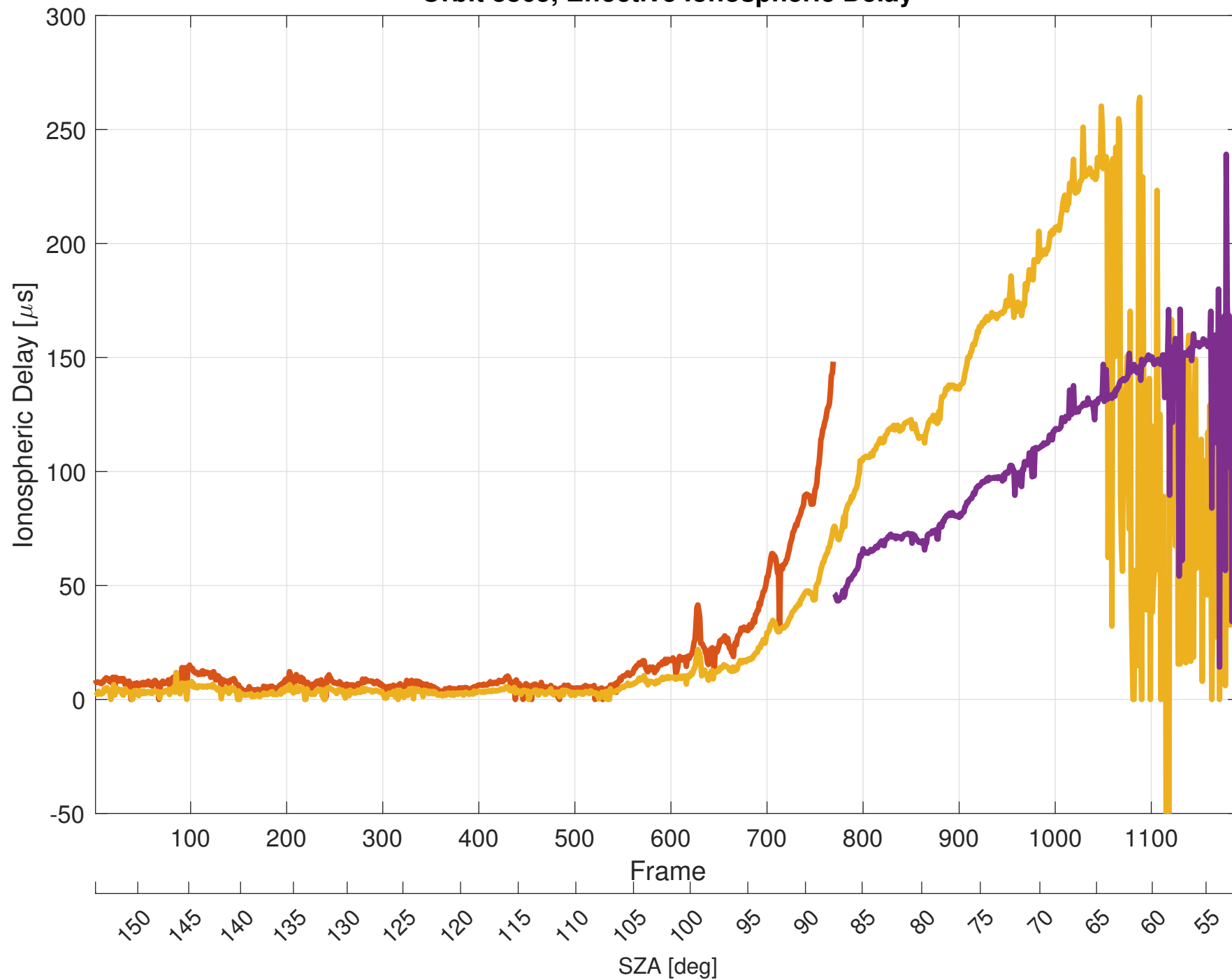
Orbit 8865, Effective Ionospheric Delay
