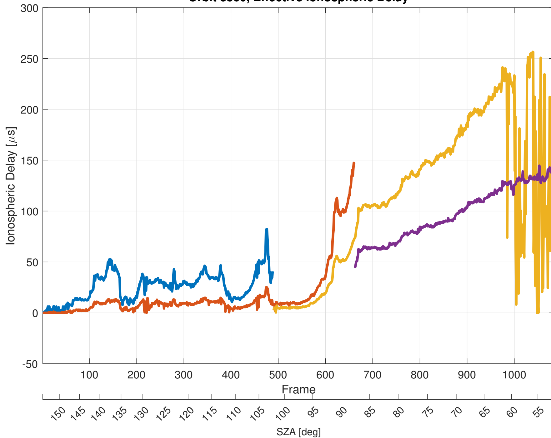
Orbit 8866, Effective Ionospheric Delay
