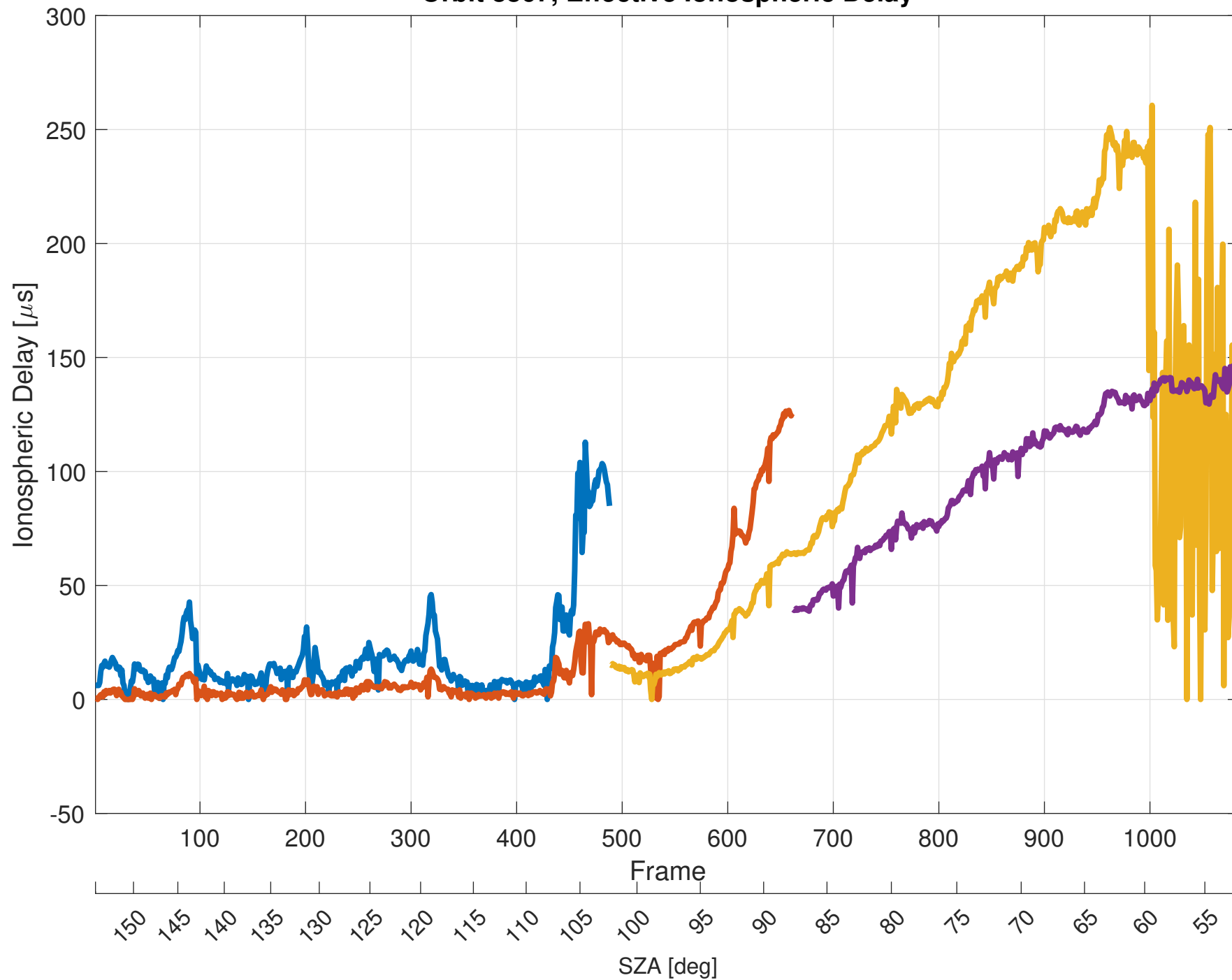
Orbit 8867, Effective Ionospheric Delay
