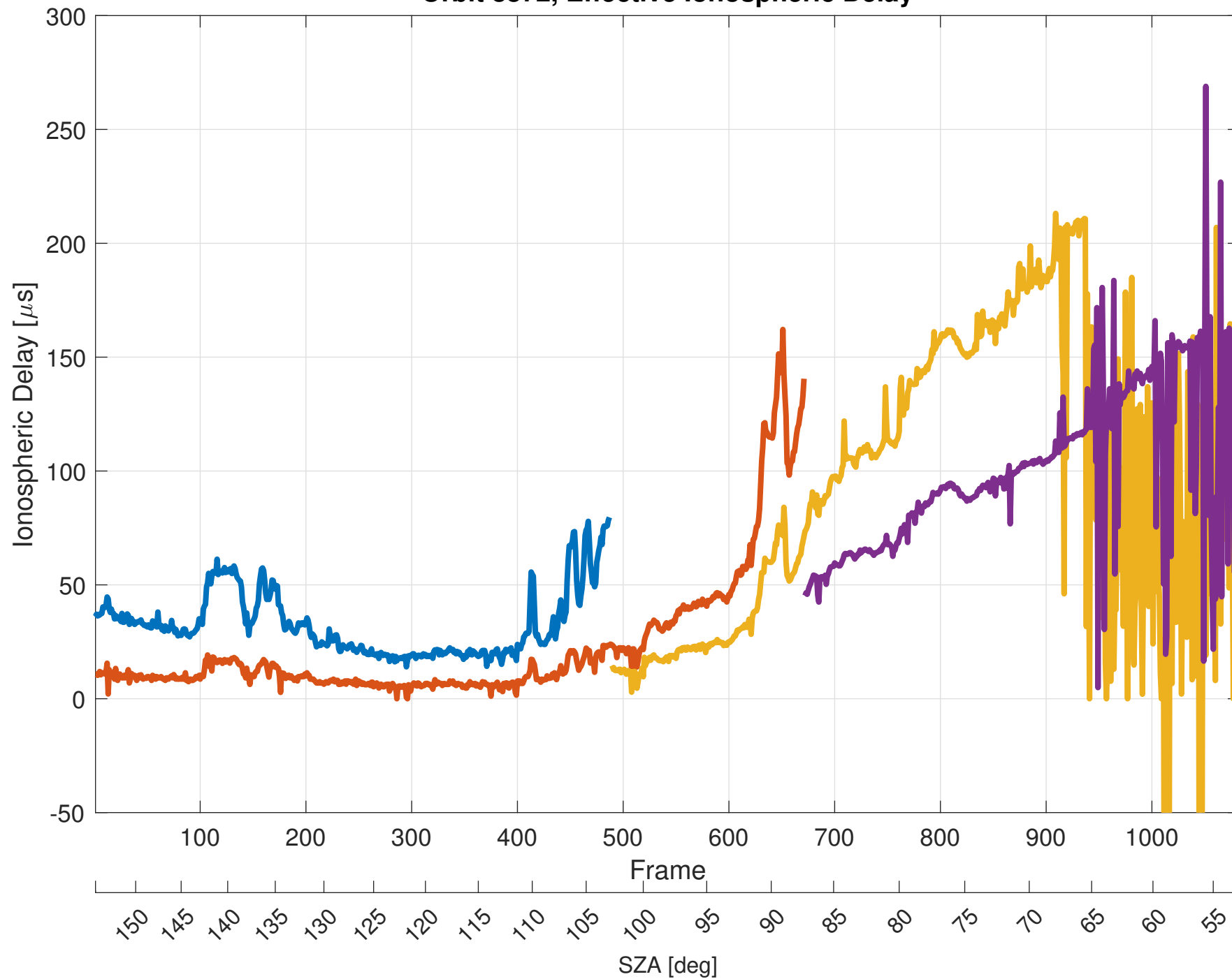
Orbit 8872, Effective Ionospheric Delay
