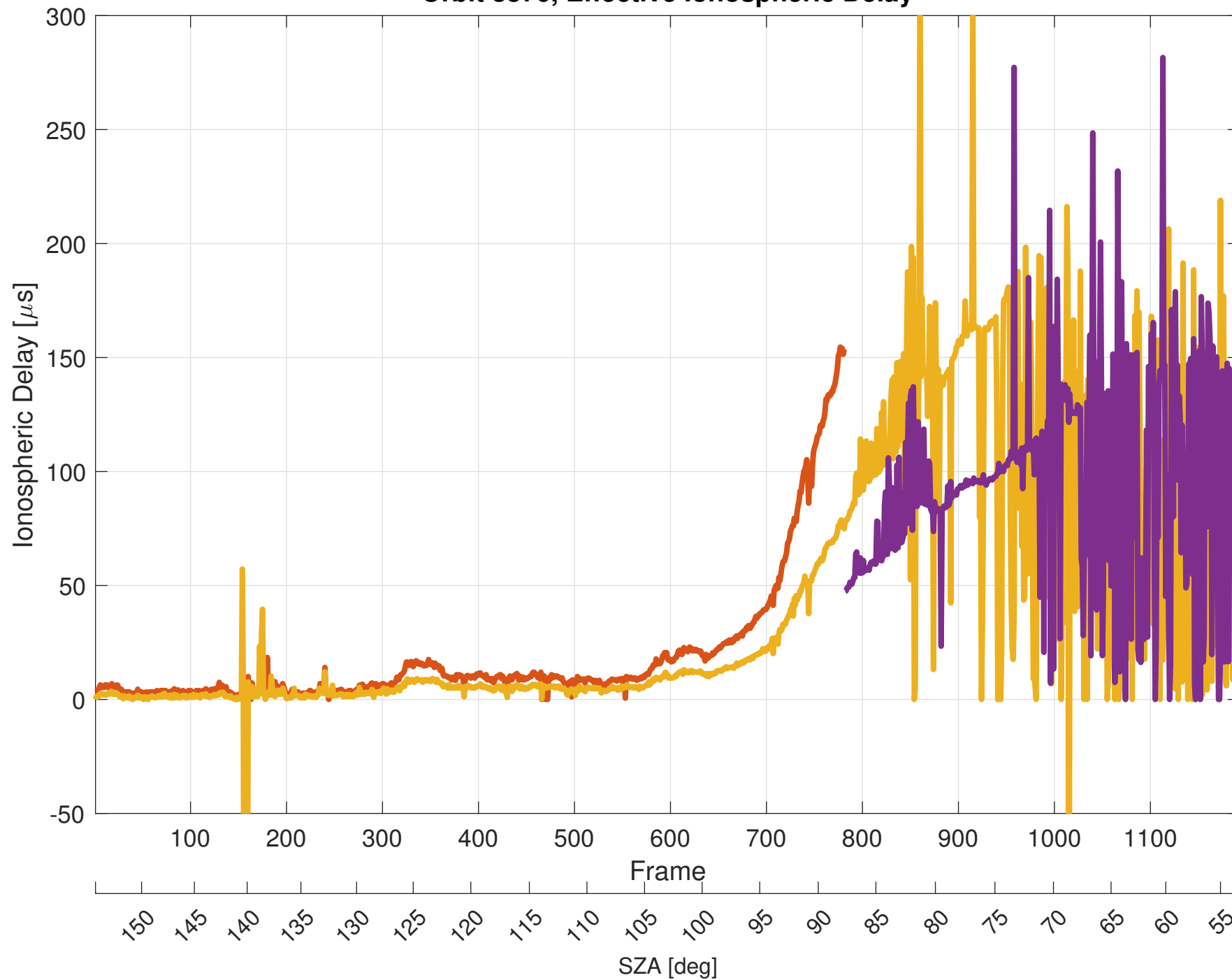
Orbit 8876, Effective Ionospheric Delay
