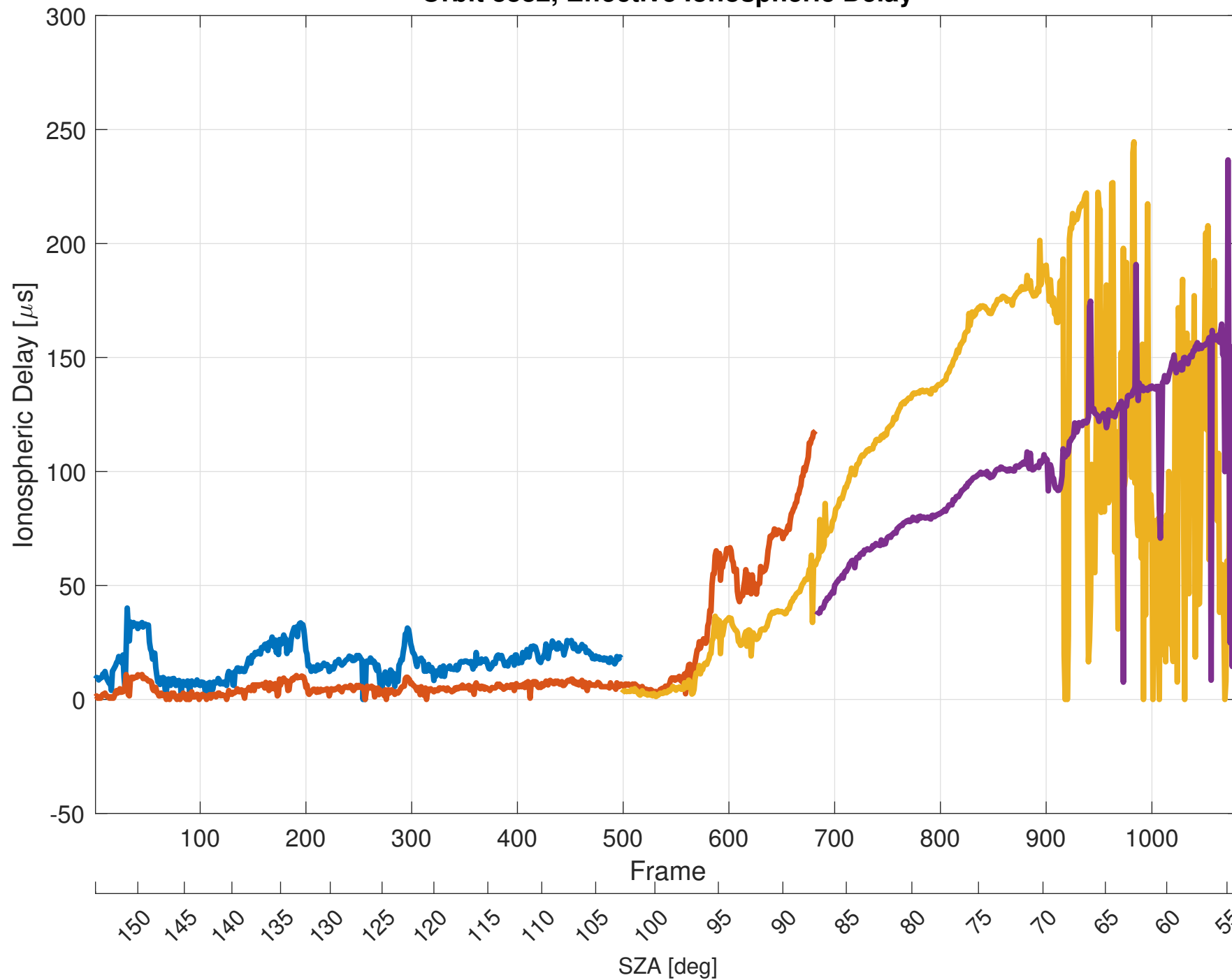
Orbit 8882, Effective Ionospheric Delay
