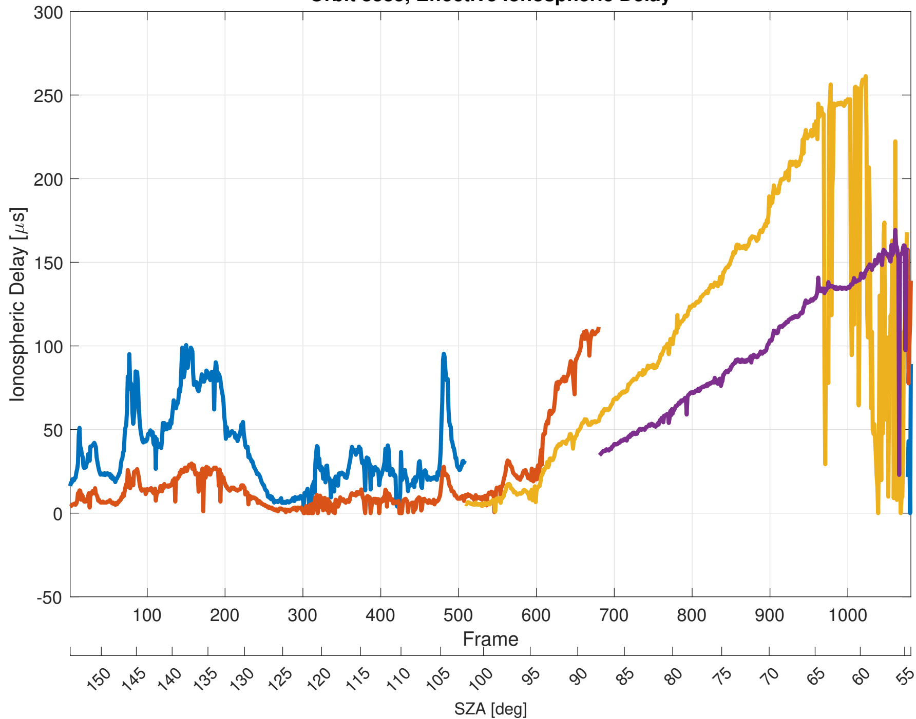
Orbit 8885, Effective Ionospheric Delay
