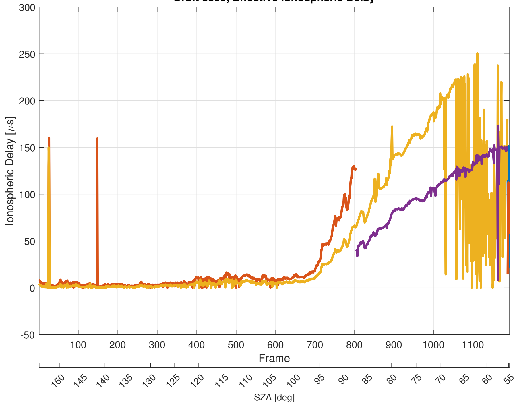
Orbit 8890, Effective Ionospheric Delay
