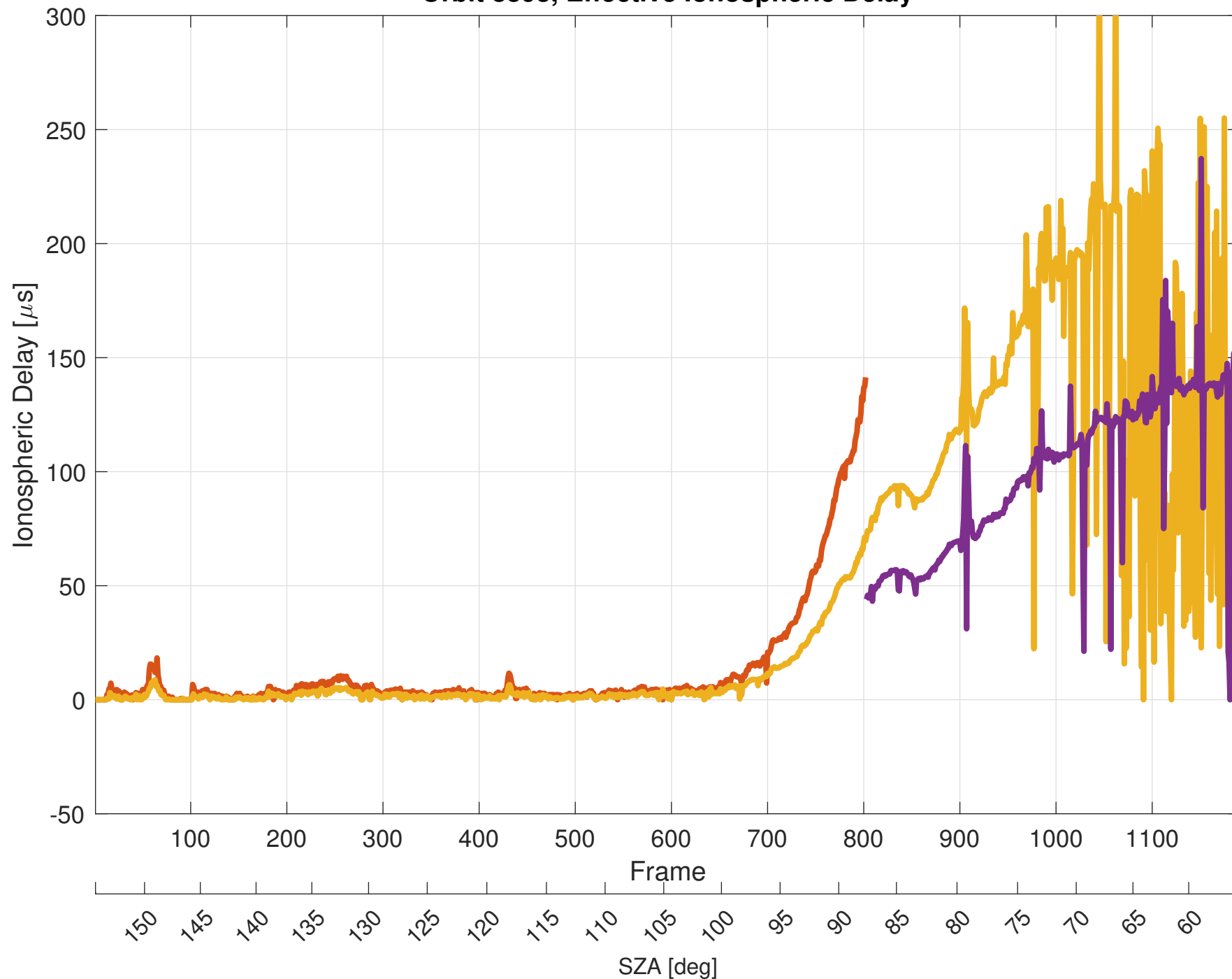
Orbit 8893, Effective Ionospheric Delay
