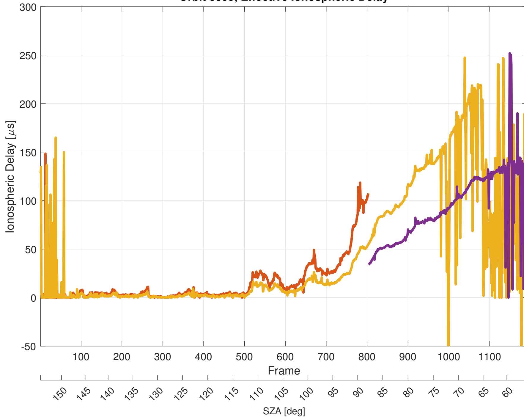
Orbit 8895, Effective Ionospheric Delay
