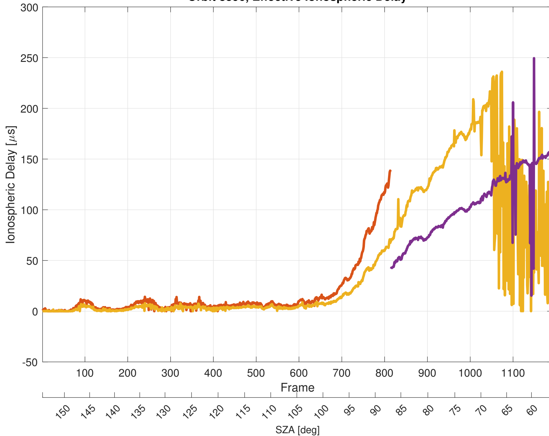
Orbit 8896, Effective Ionospheric Delay
