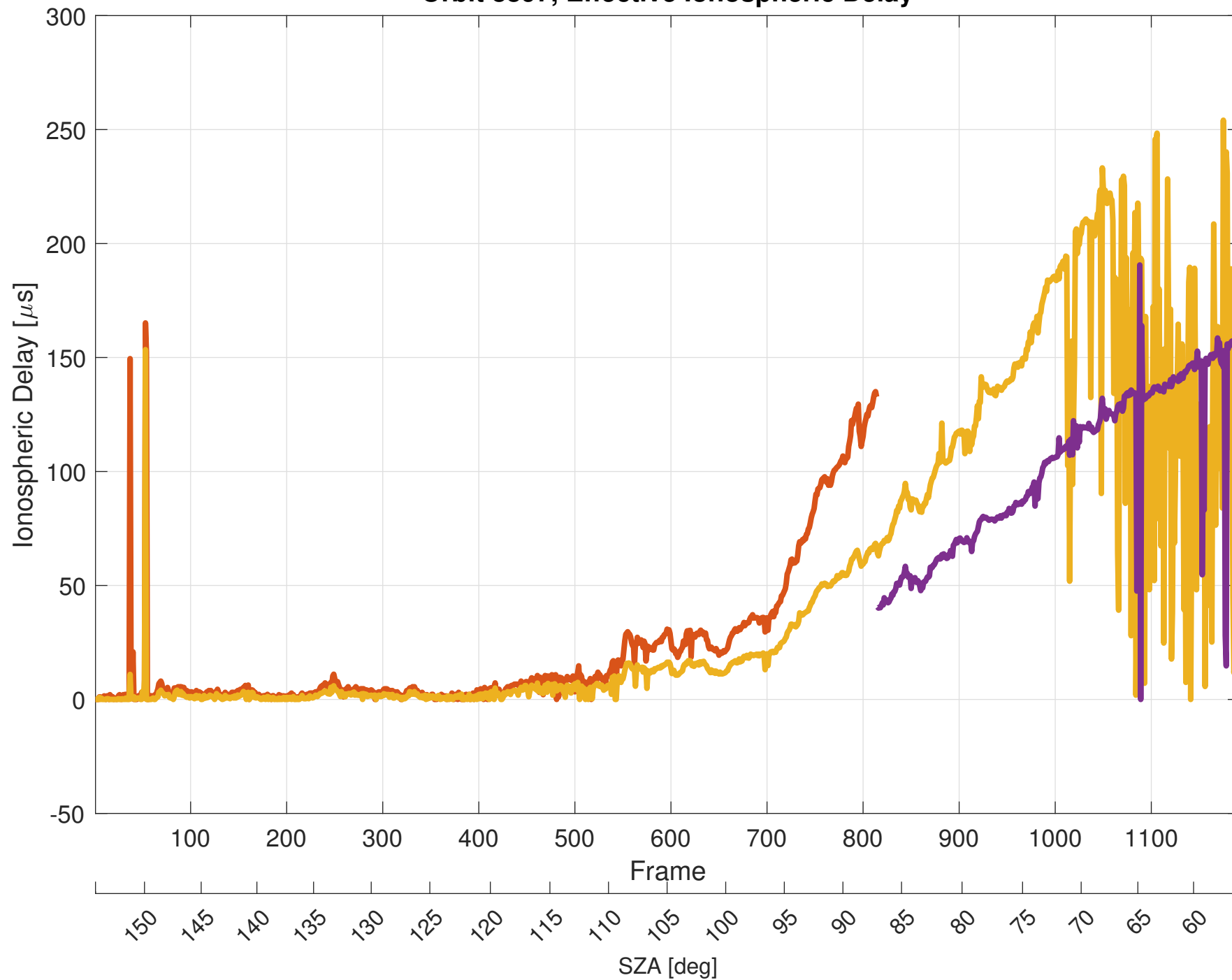
Orbit 8897, Effective Ionospheric Delay
