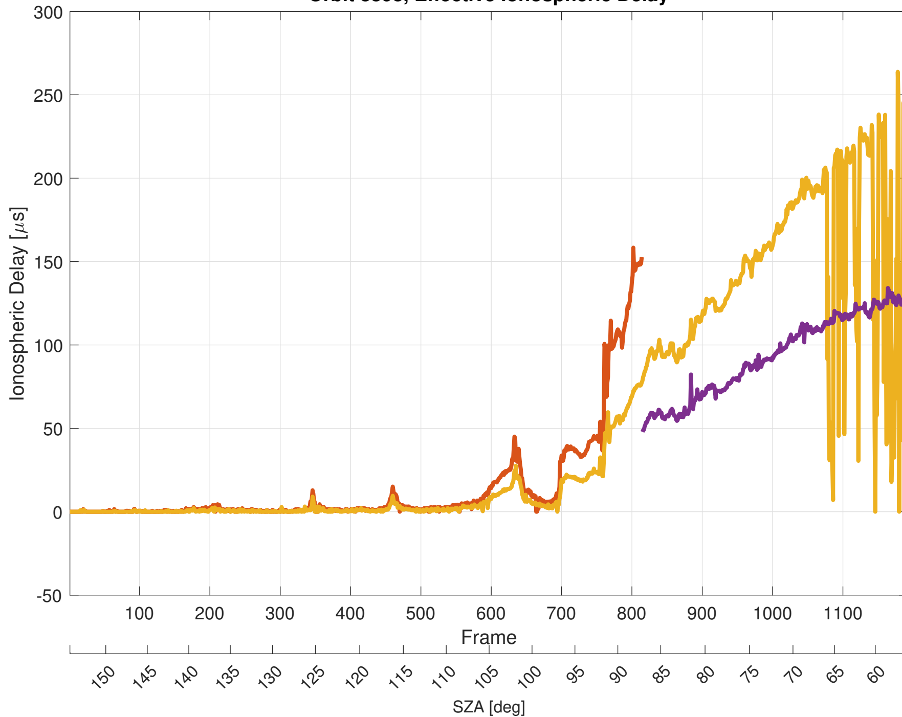
Orbit 8898, Effective Ionospheric Delay
