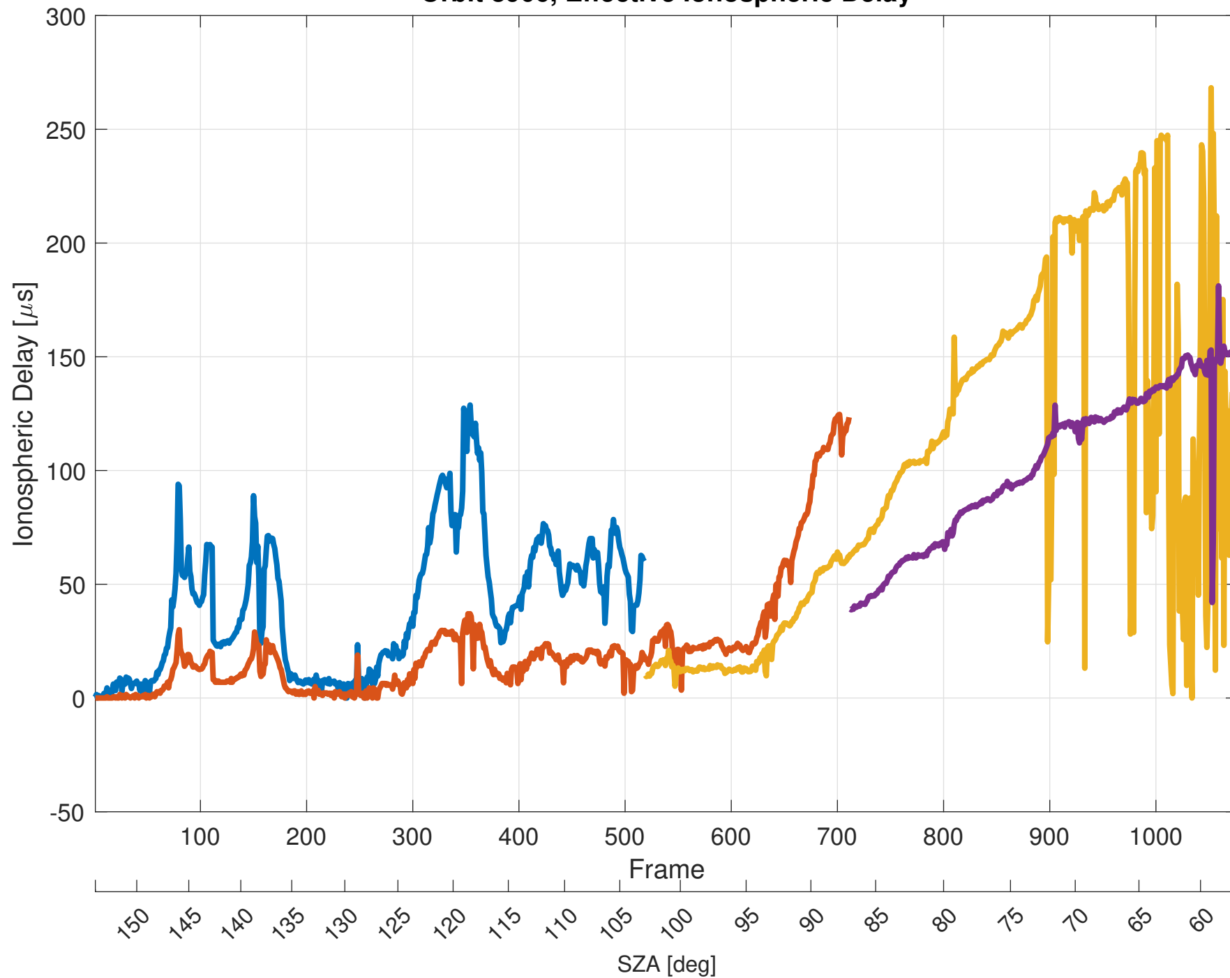
Orbit 8906, Effective Ionospheric Delay
