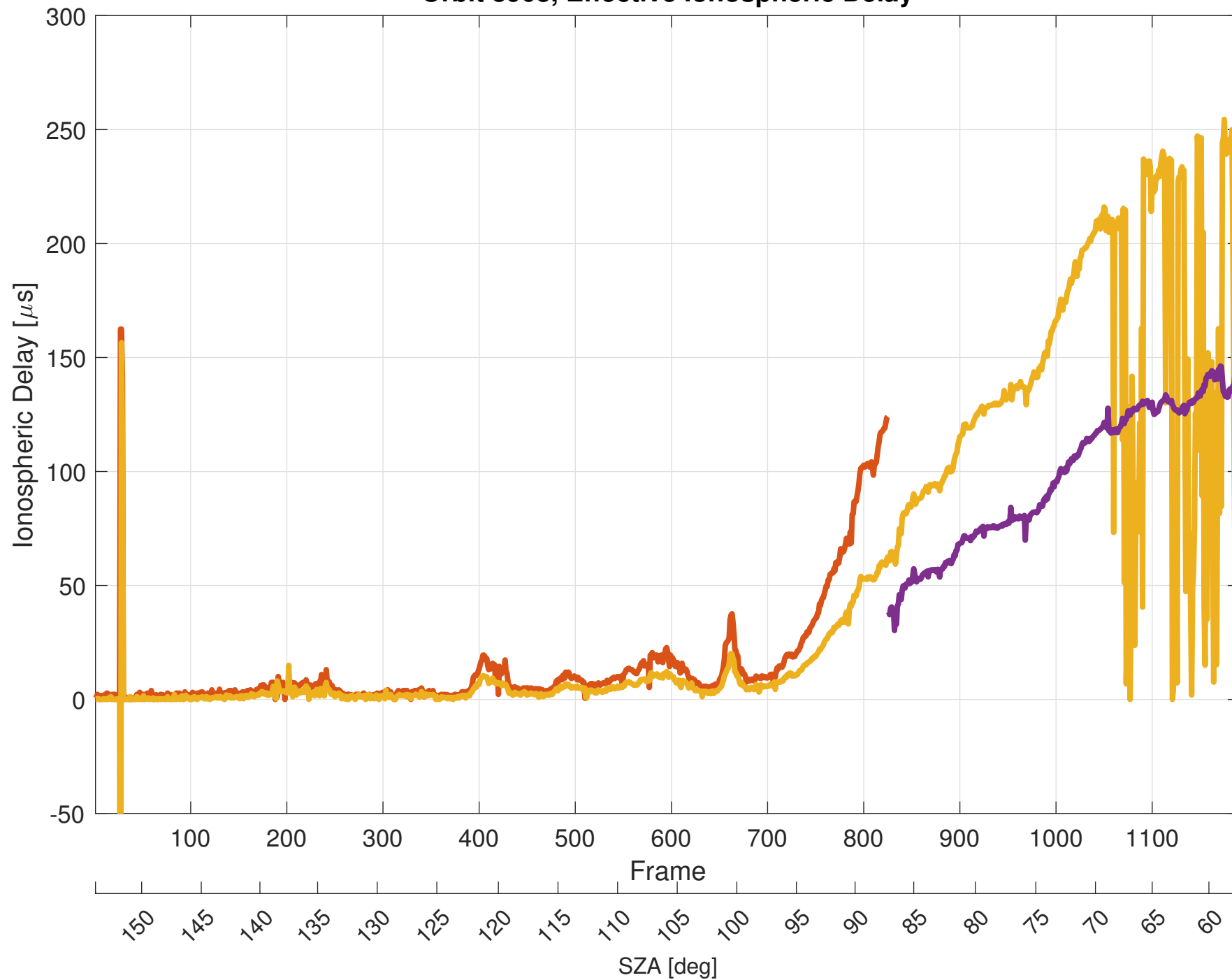
Orbit 8908, Effective Ionospheric Delay
