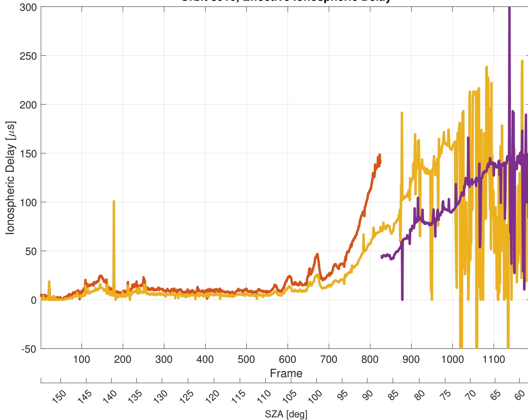
Orbit 8910, Effective Ionospheric Delay
