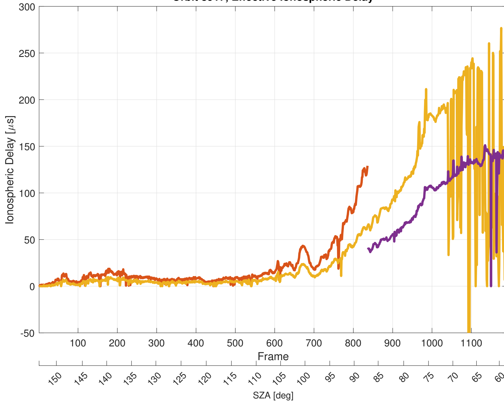
Orbit 8917, Effective Ionospheric Delay
