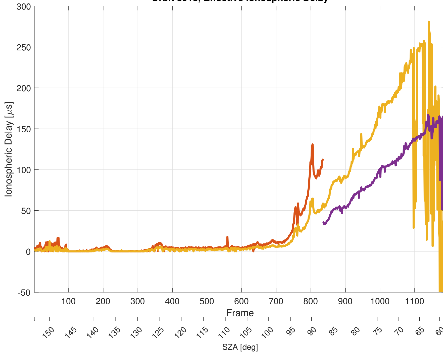
Orbit 8918, Effective Ionospheric Delay
