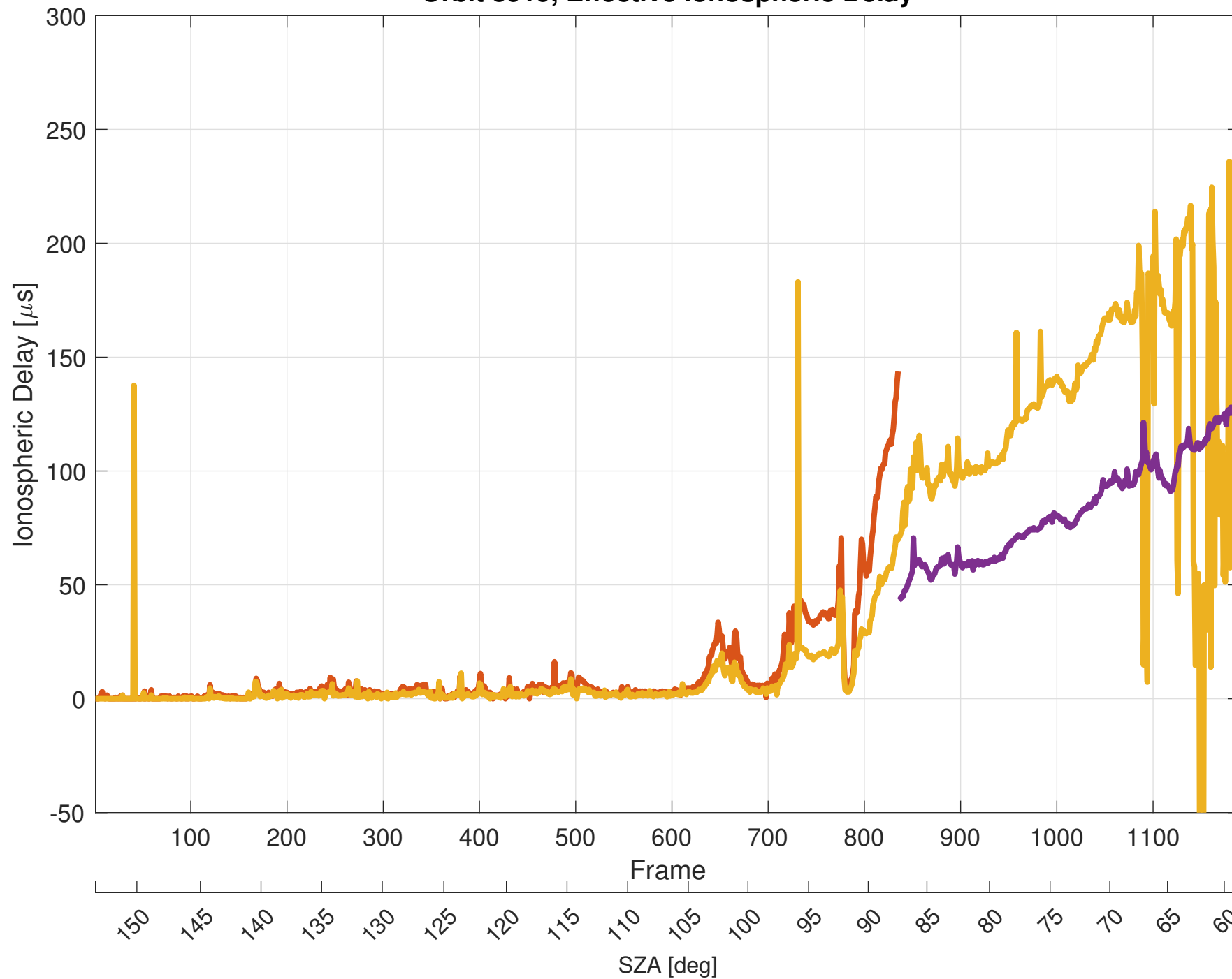
Orbit 8919, Effective Ionospheric Delay
