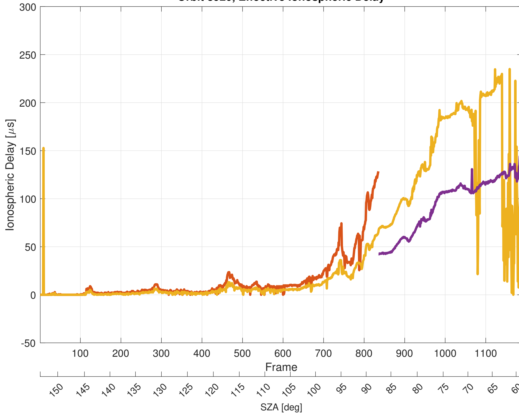
Orbit 8920, Effective Ionospheric Delay
