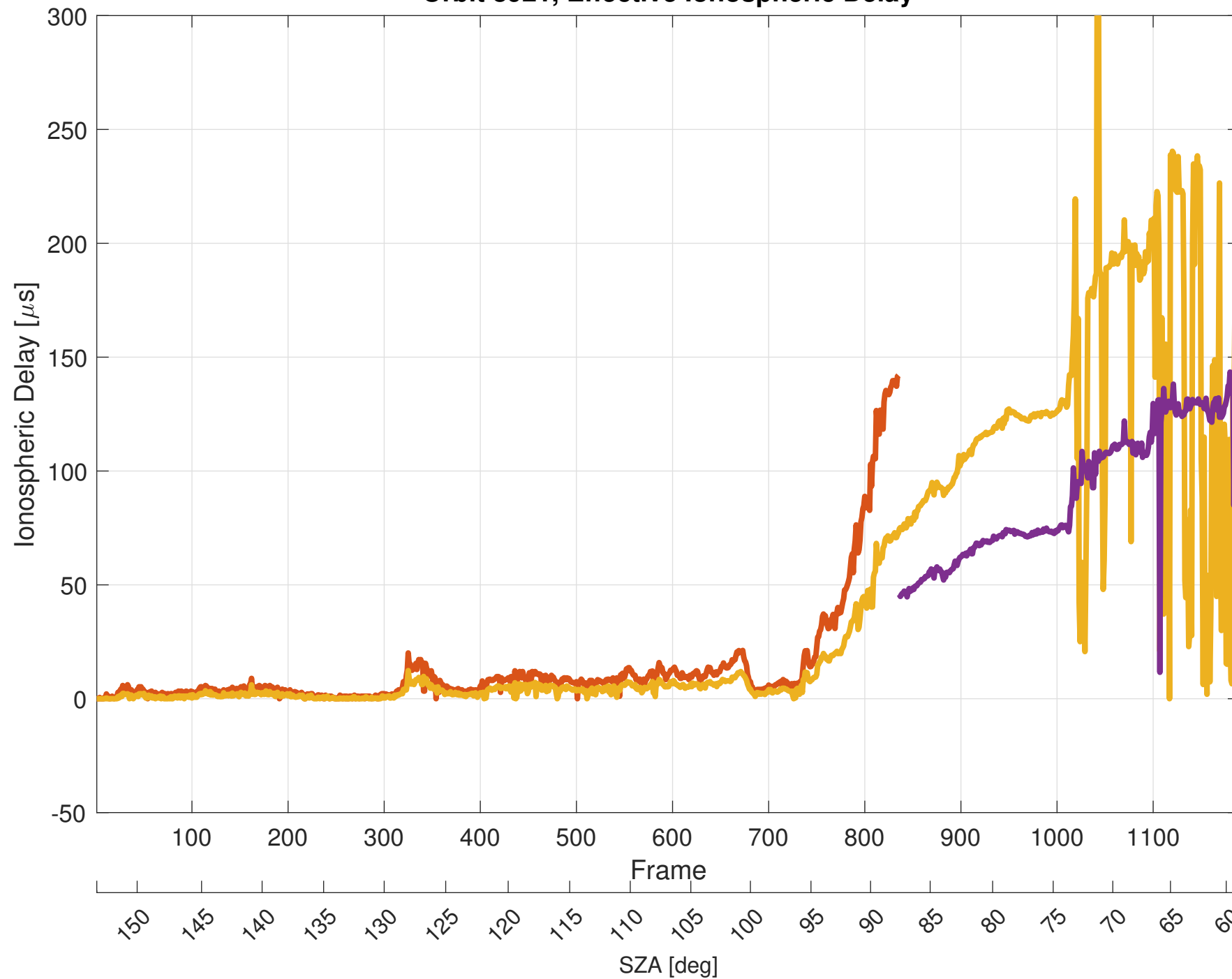
Orbit 8921, Effective Ionospheric Delay
