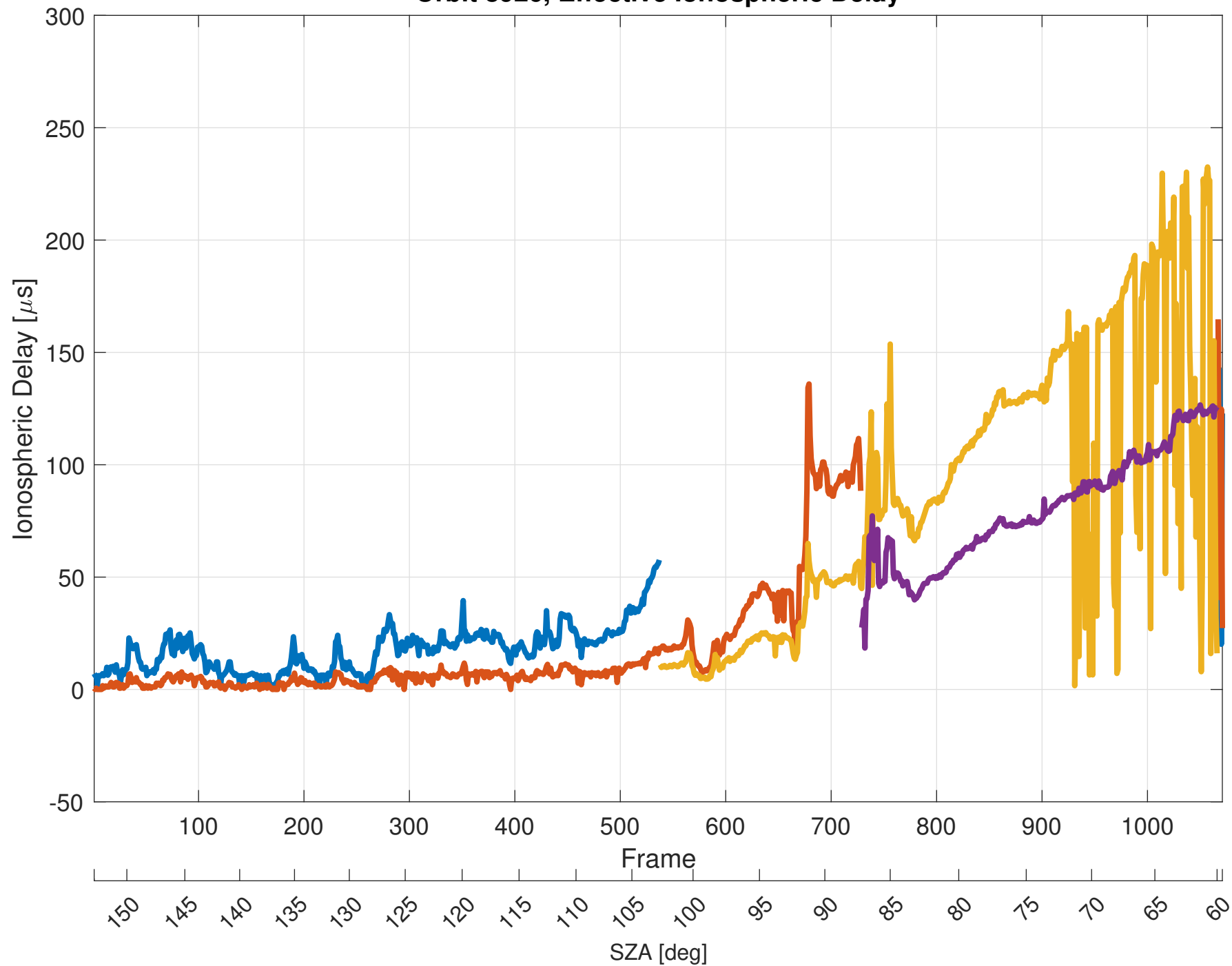
Orbit 8926, Effective Ionospheric Delay
