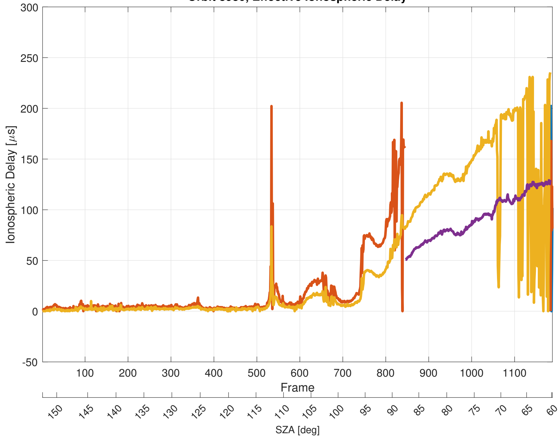
Orbit 8930, Effective Ionospheric Delay
