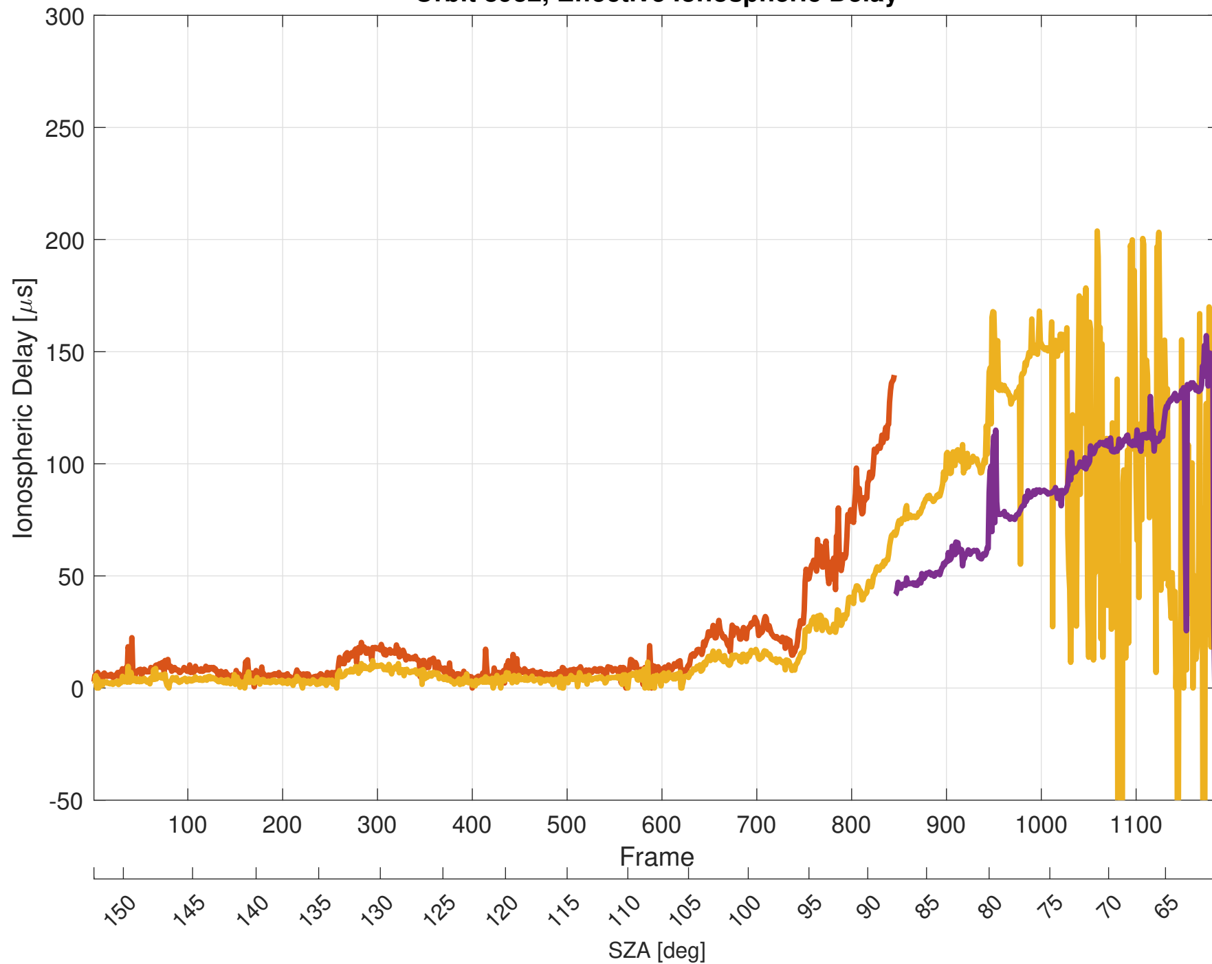
Orbit 8932, Effective Ionospheric Delay
