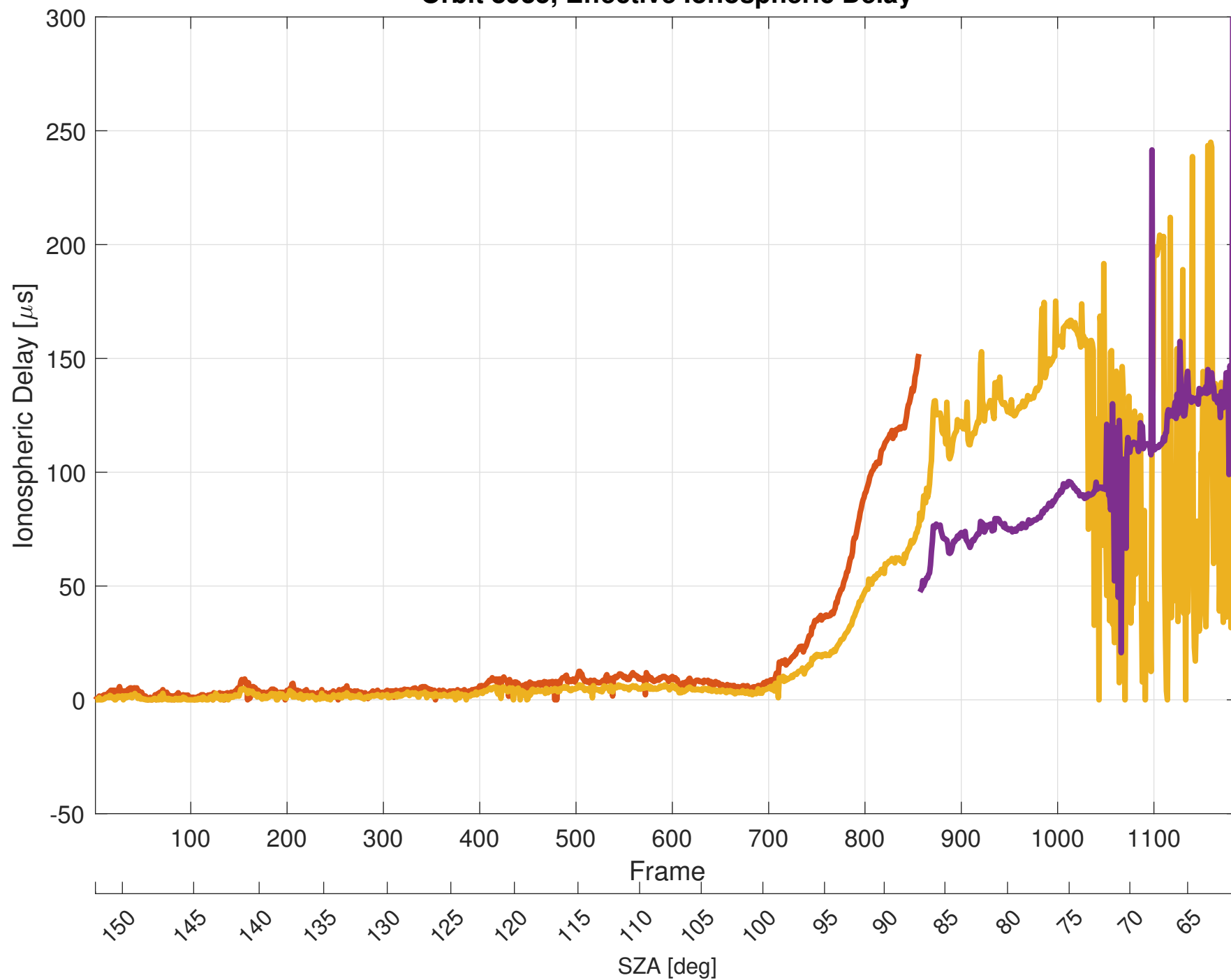
Orbit 8935, Effective Ionospheric Delay
