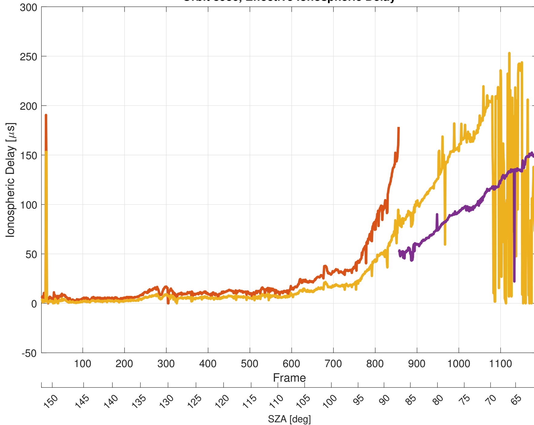
Orbit 8936, Effective Ionospheric Delay
