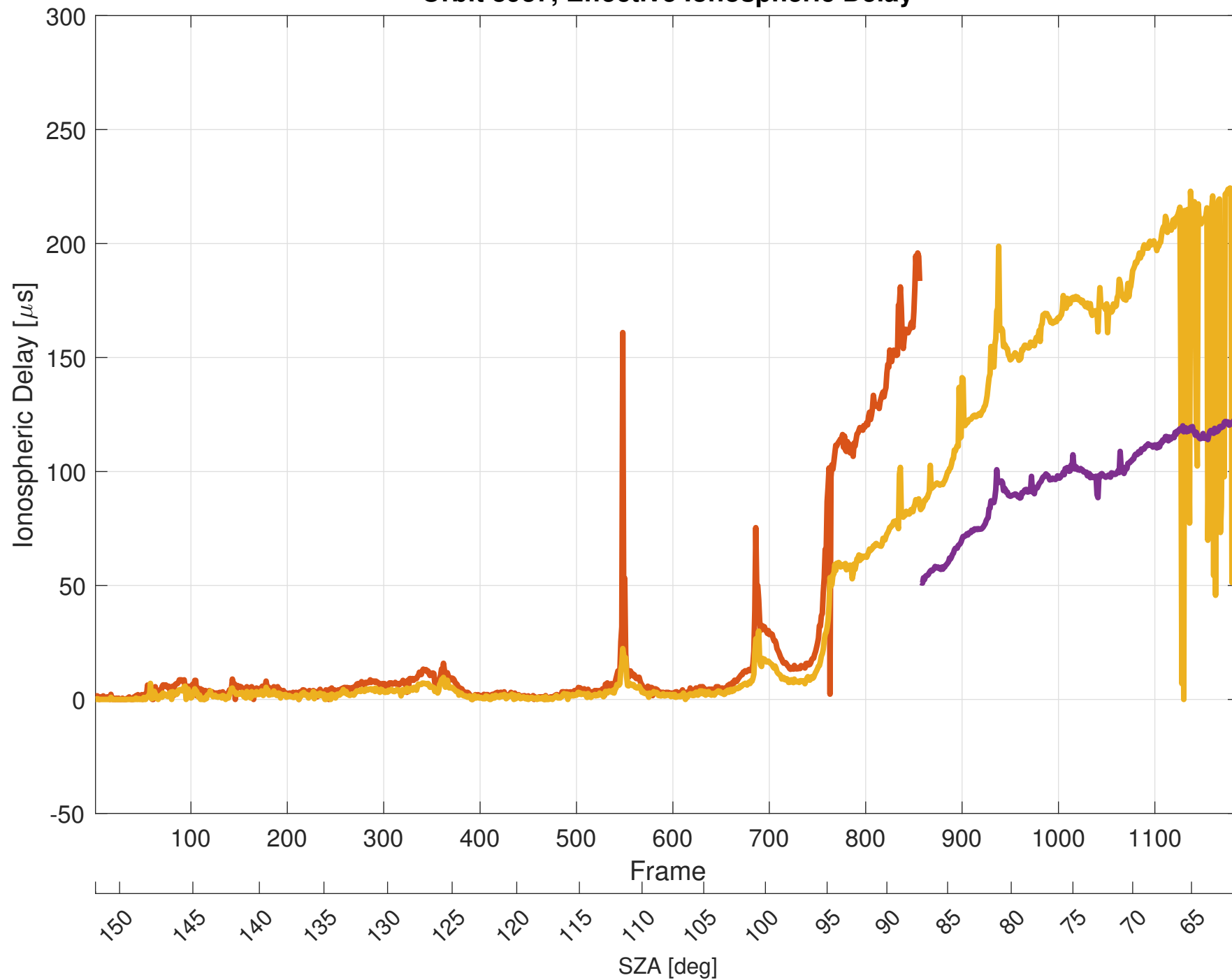
Orbit 8937, Effective Ionospheric Delay
