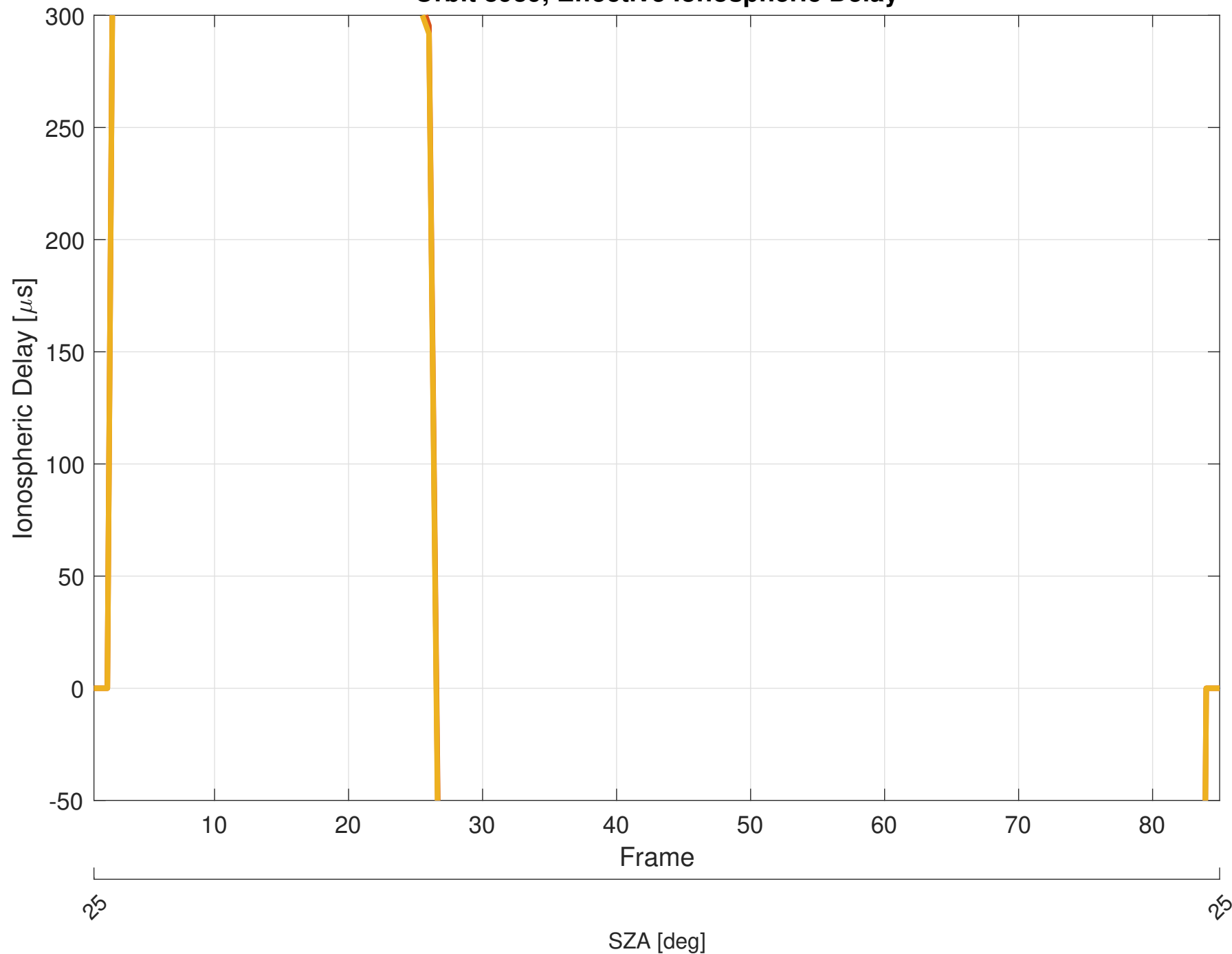
Orbit 8939, Effective Ionospheric Delay
