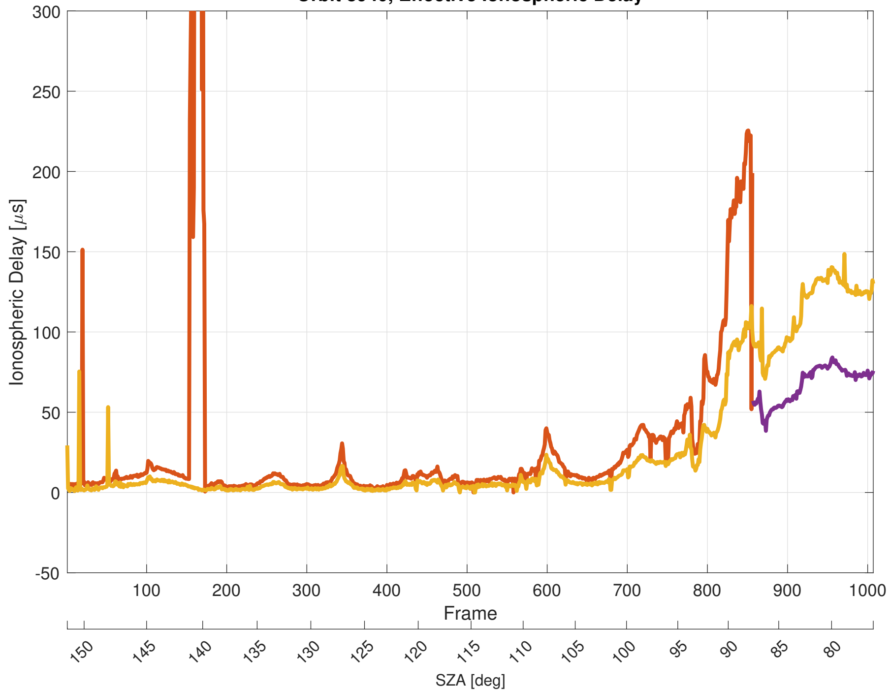
Orbit 8940, Effective Ionospheric Delay
