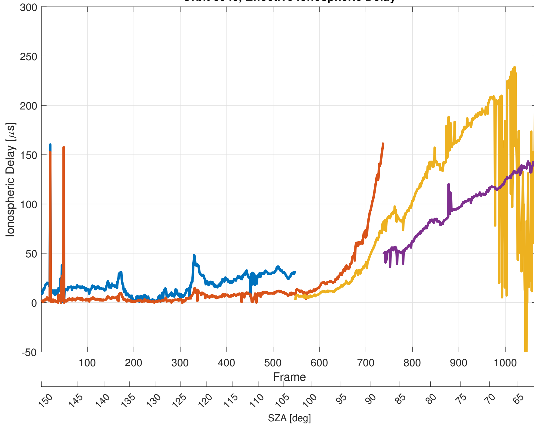
Orbit 8943, Effective Ionospheric Delay
