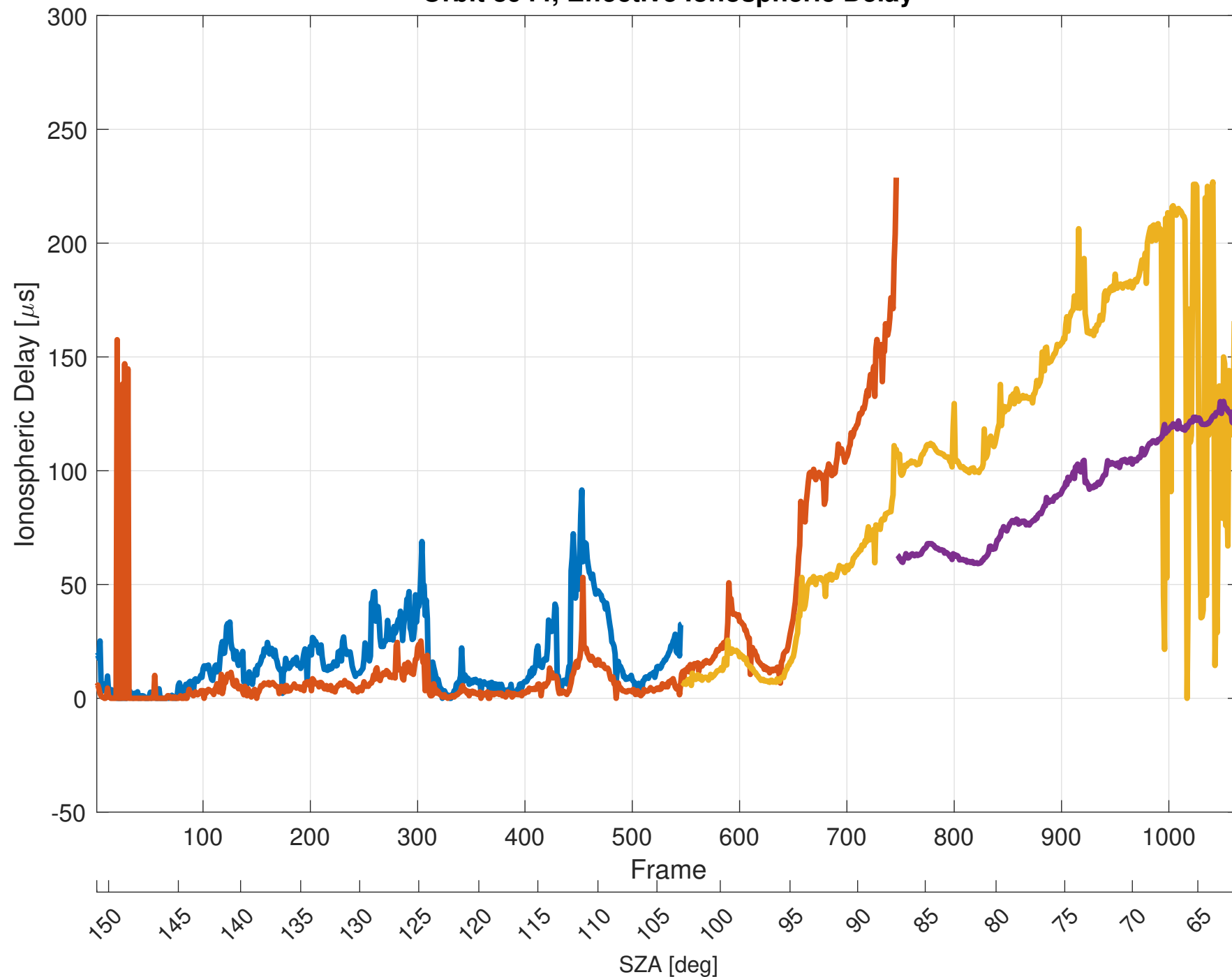
Orbit 8944, Effective Ionospheric Delay
