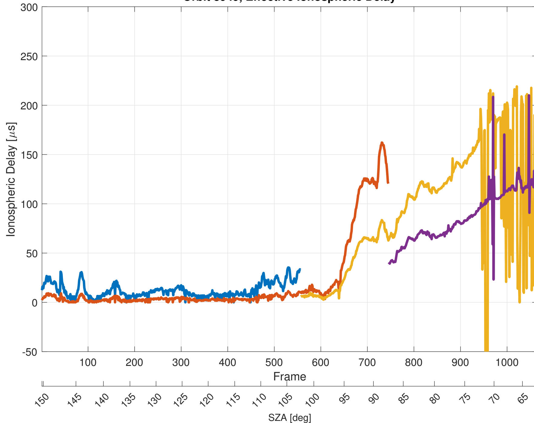
Orbit 8949, Effective Ionospheric Delay
