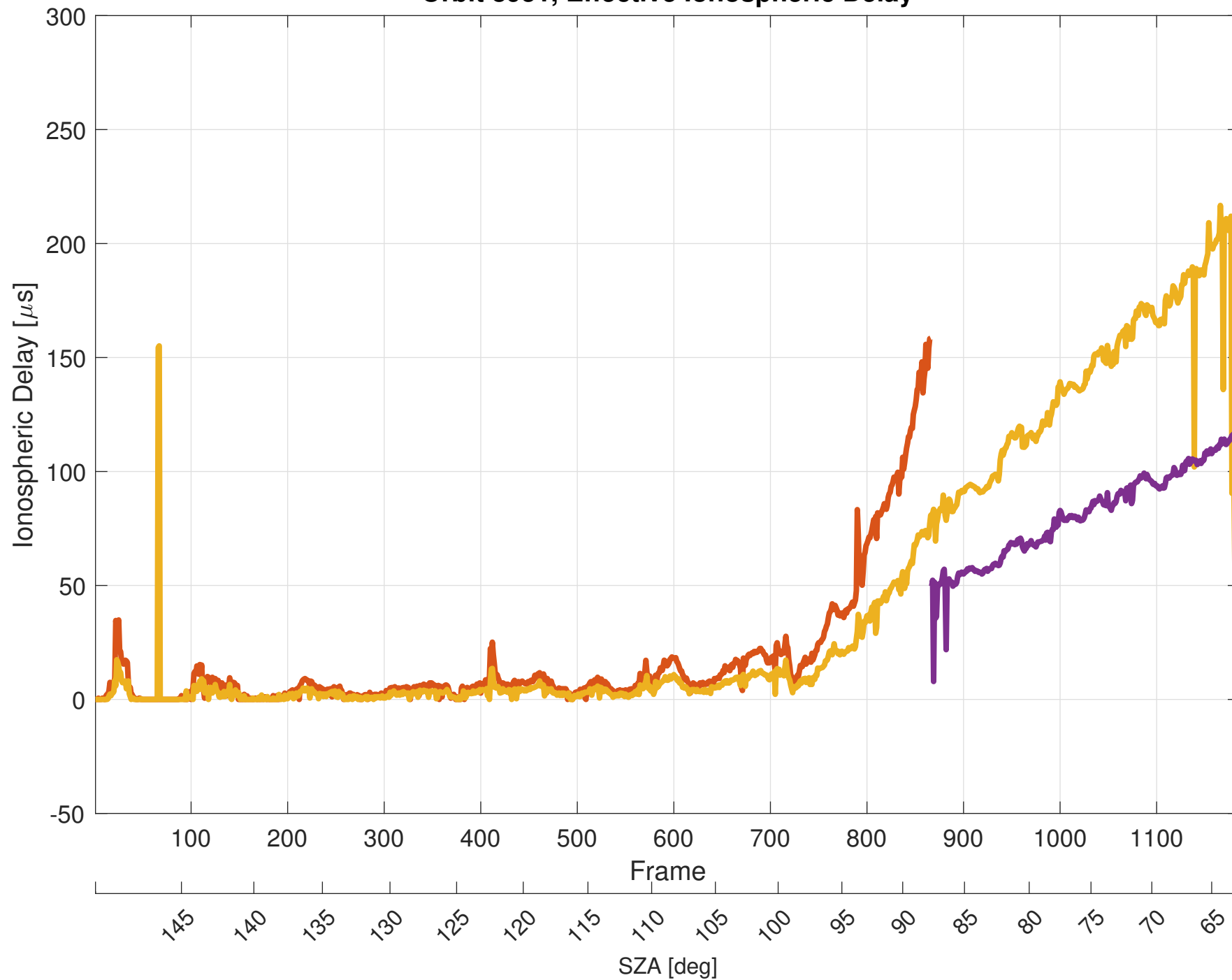
Orbit 8951, Effective Ionospheric Delay
